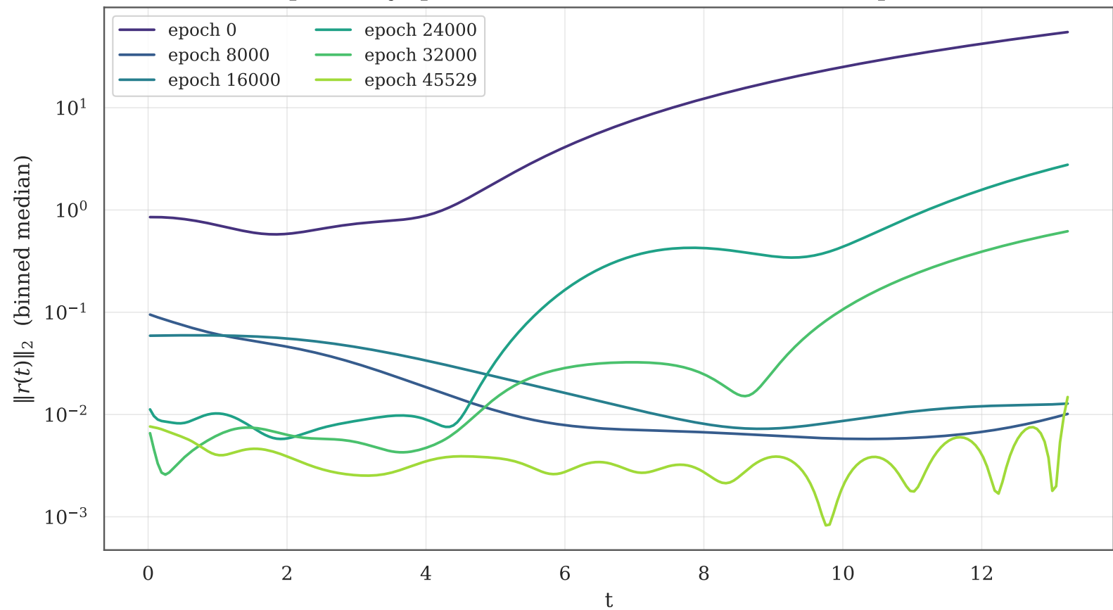
Residual profile by epoch — 4x60 tanh, hard IC, 39793 LHS points, causal
