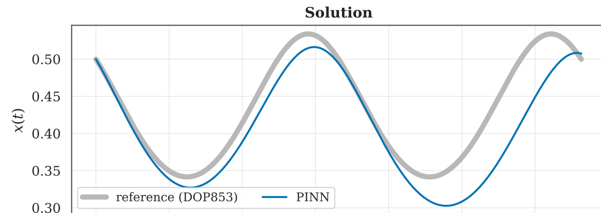
PINN solution vs reference — 4x60 tanh, hard IC, 39793 LHS points, causal
