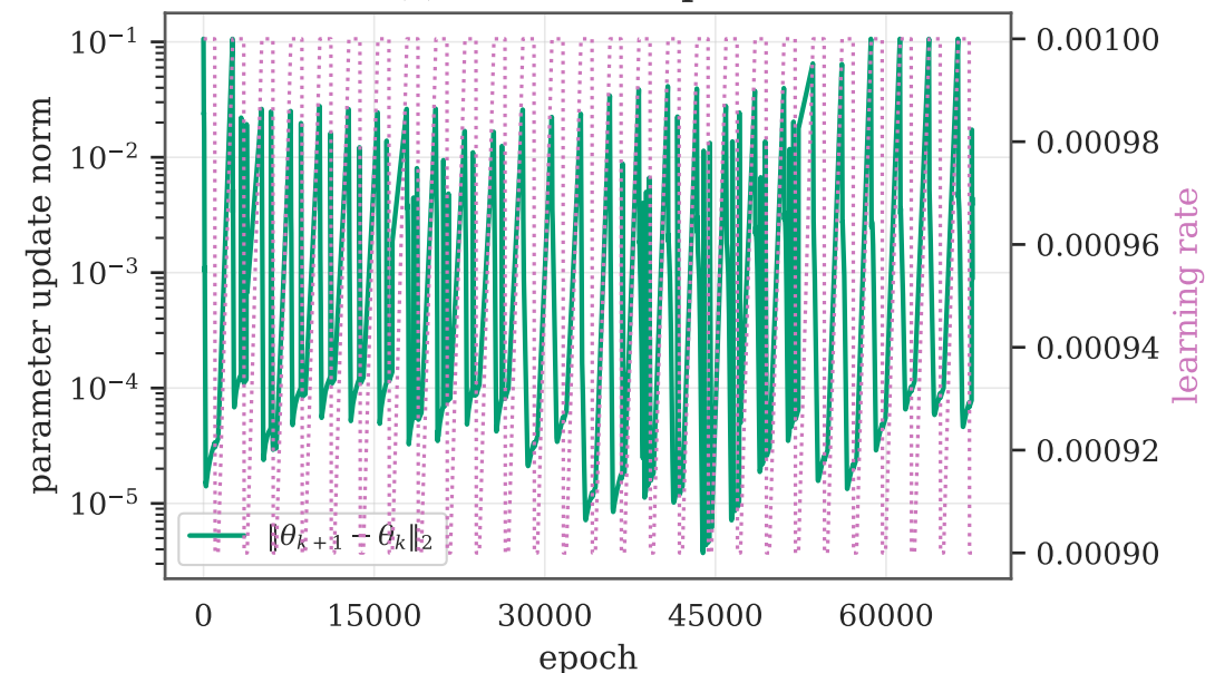
(c) Effective step size
