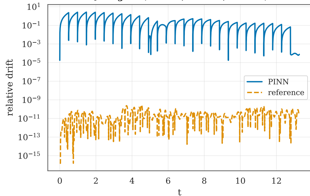
I_1 weights (+0.904, +0.226, +0.363)
