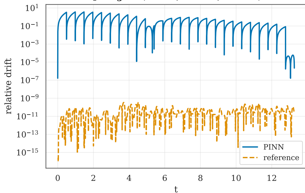
I_2 weights (-0.424, +0.363, +0.830)
