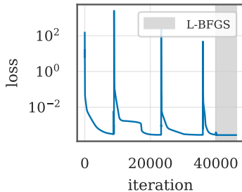
Training loss
