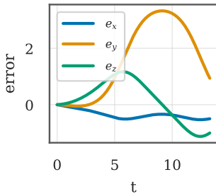
Error, RMSE 2.237
