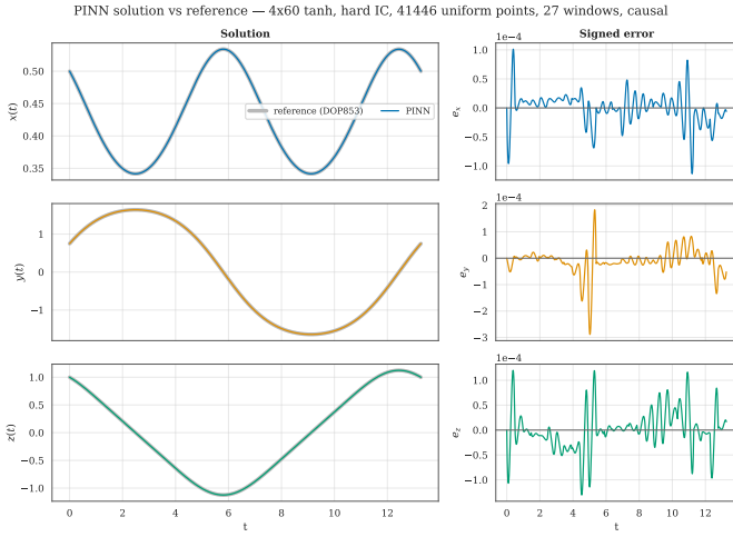
Fig. 3. Seed-0 windowed PINN against DOP853. The prediction overlaps the reference, and the signed errors stay below 3 \times 10^{-4} .
