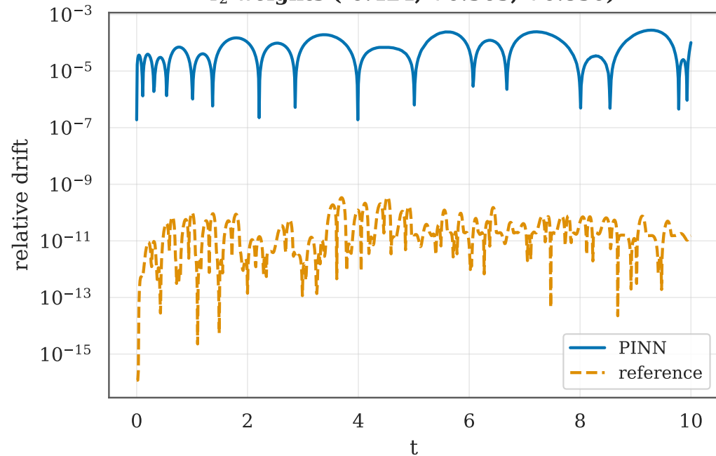
I_2 weights (-0.424, +0.363, +0.830)
