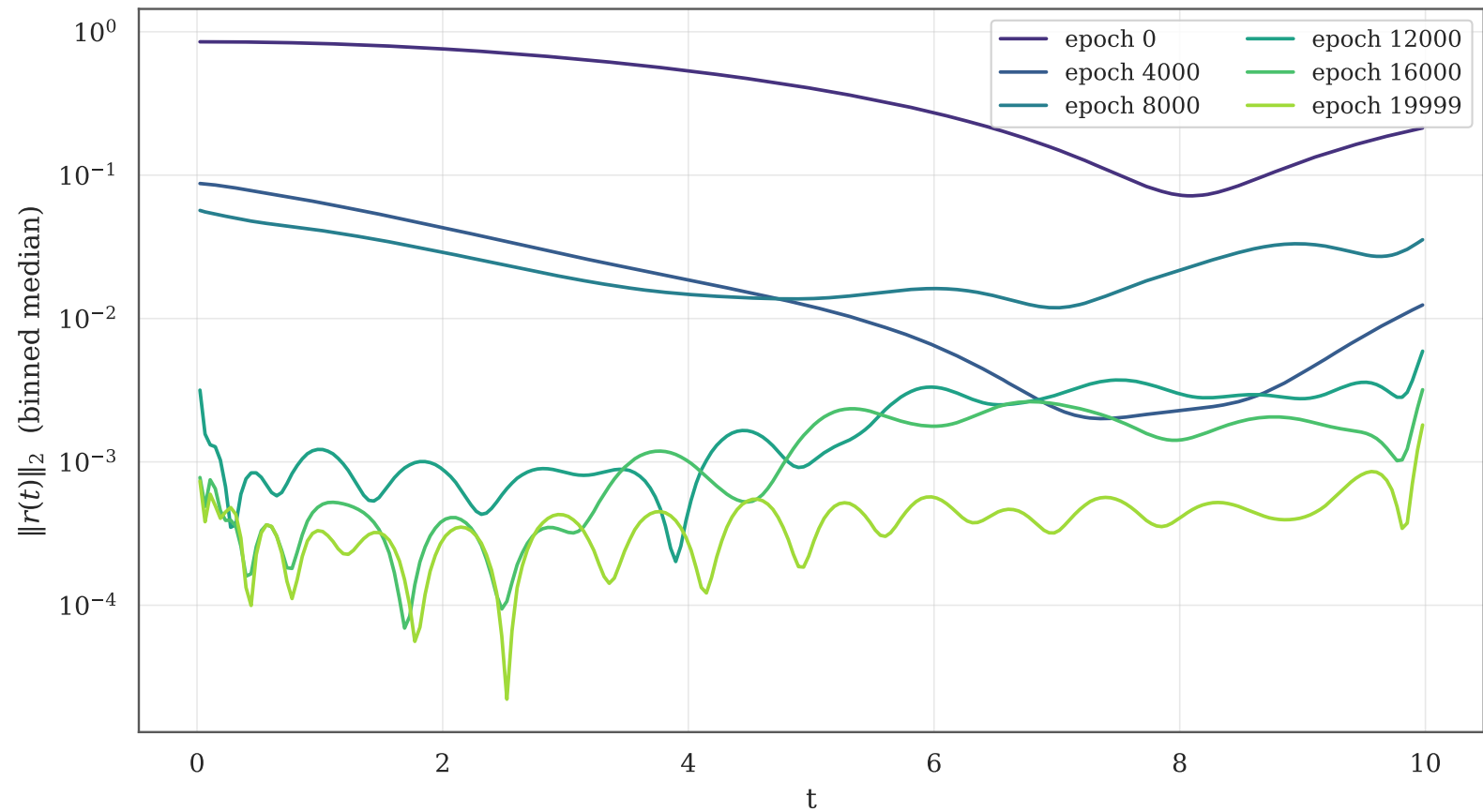
Residual profile by epoch — 4x60 tanh, hard IC, causal, 3000 LHS points
