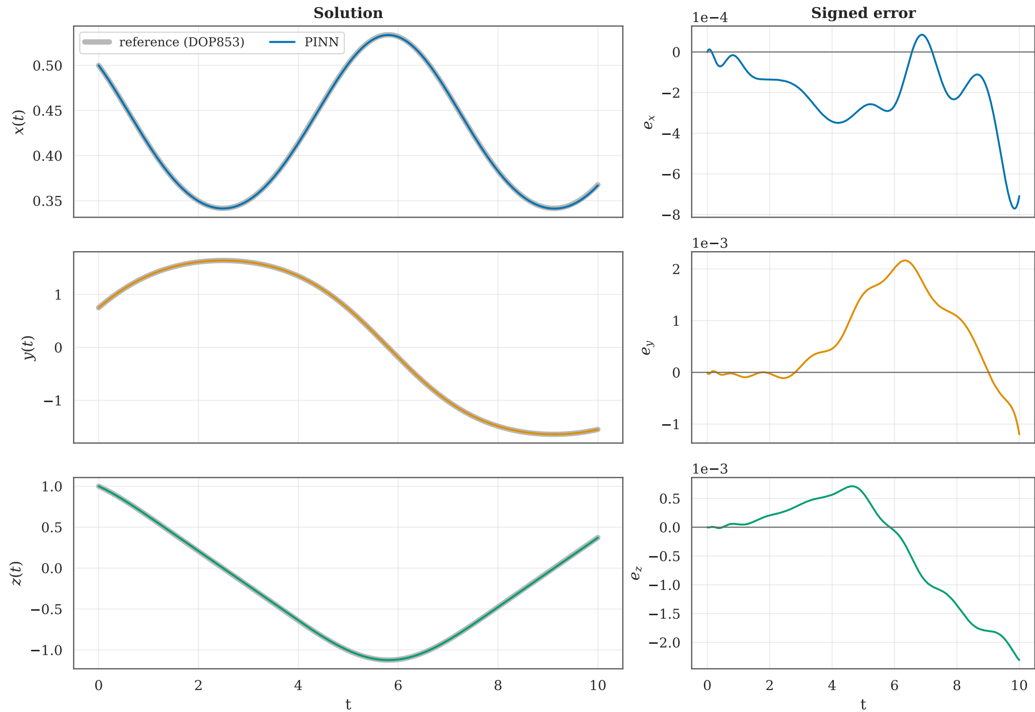
PINN solution vs reference — 4x60 tanh, hard IC, causal, 3000 LHS points
