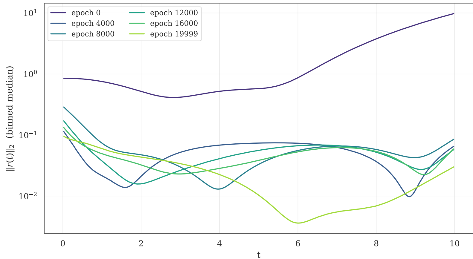
Residual profile by epoch — 4x60 tanh, hard IC, sequential walk, 3000 LHS points
