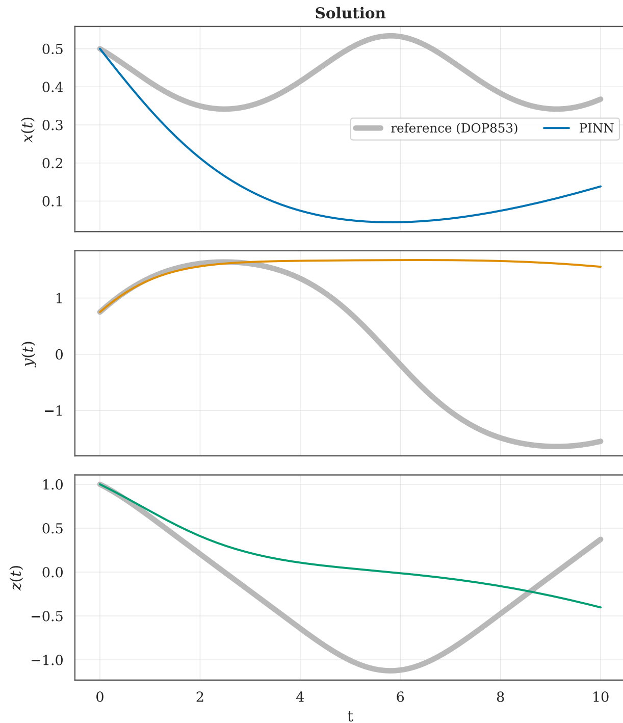
PINN solution vs reference — 4x60 tanh, hard IC, sequential walk, 3000 LHS points
