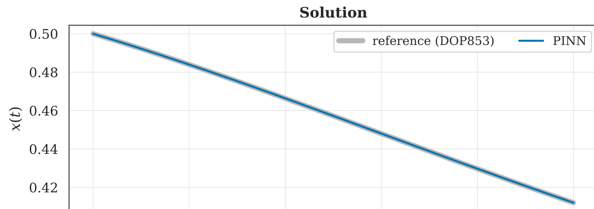
PINN solution vs reference — 5x50 tanh, hard IC, 3000 LHS points
