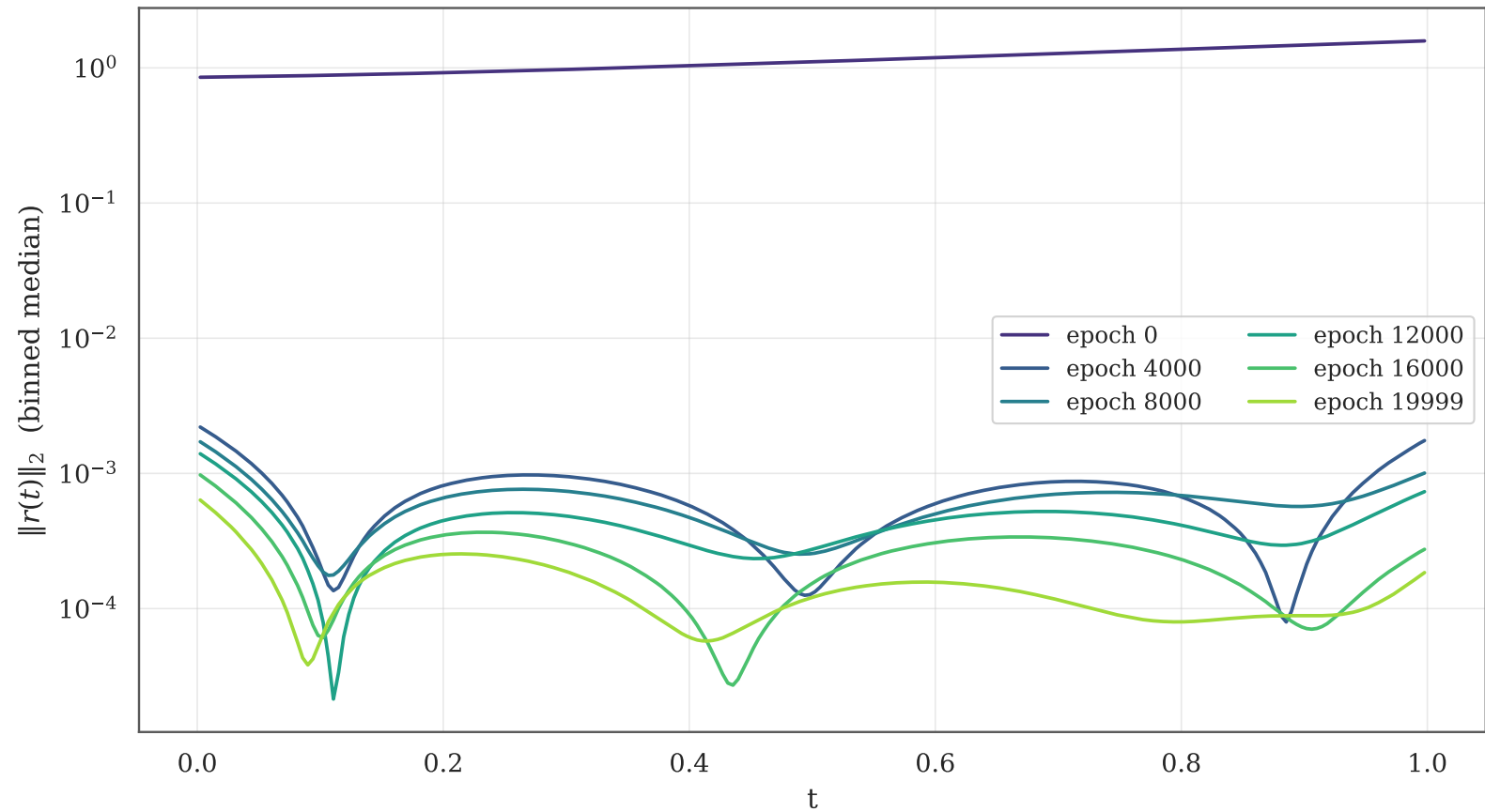
Residual profile by epoch — 3x50 tanh, hard IC, 3000 LHS points
