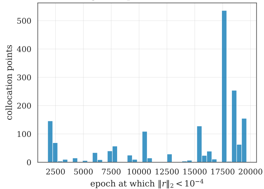
(a) Convergence epoch (1196 never reached)
