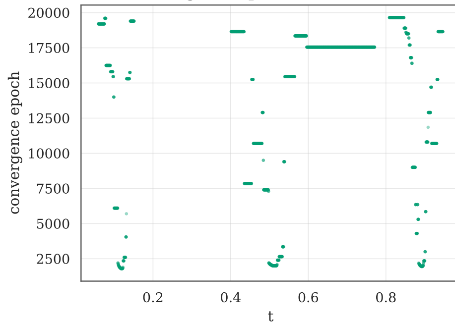
(b) Convergence epoch across the domain
