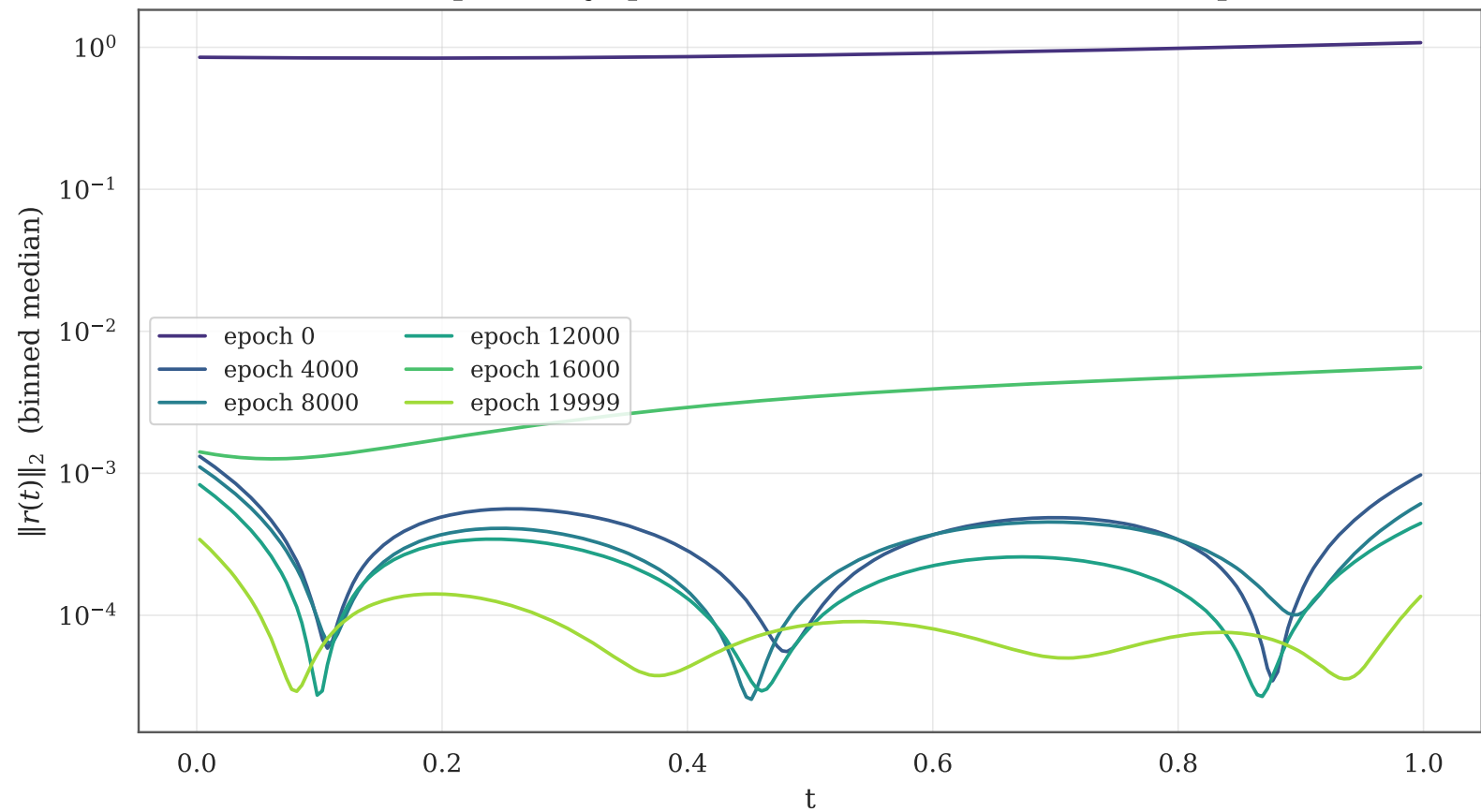
Residual profile by epoch — 4x50 tanh, hard IC, 3000 LHS points
