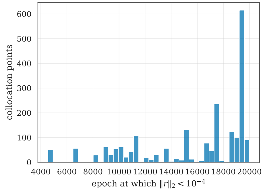
(a) Convergence epoch (904 never reached)
