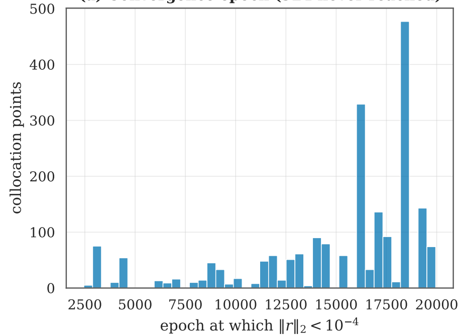
(a) Convergence epoch (924 never reached)
