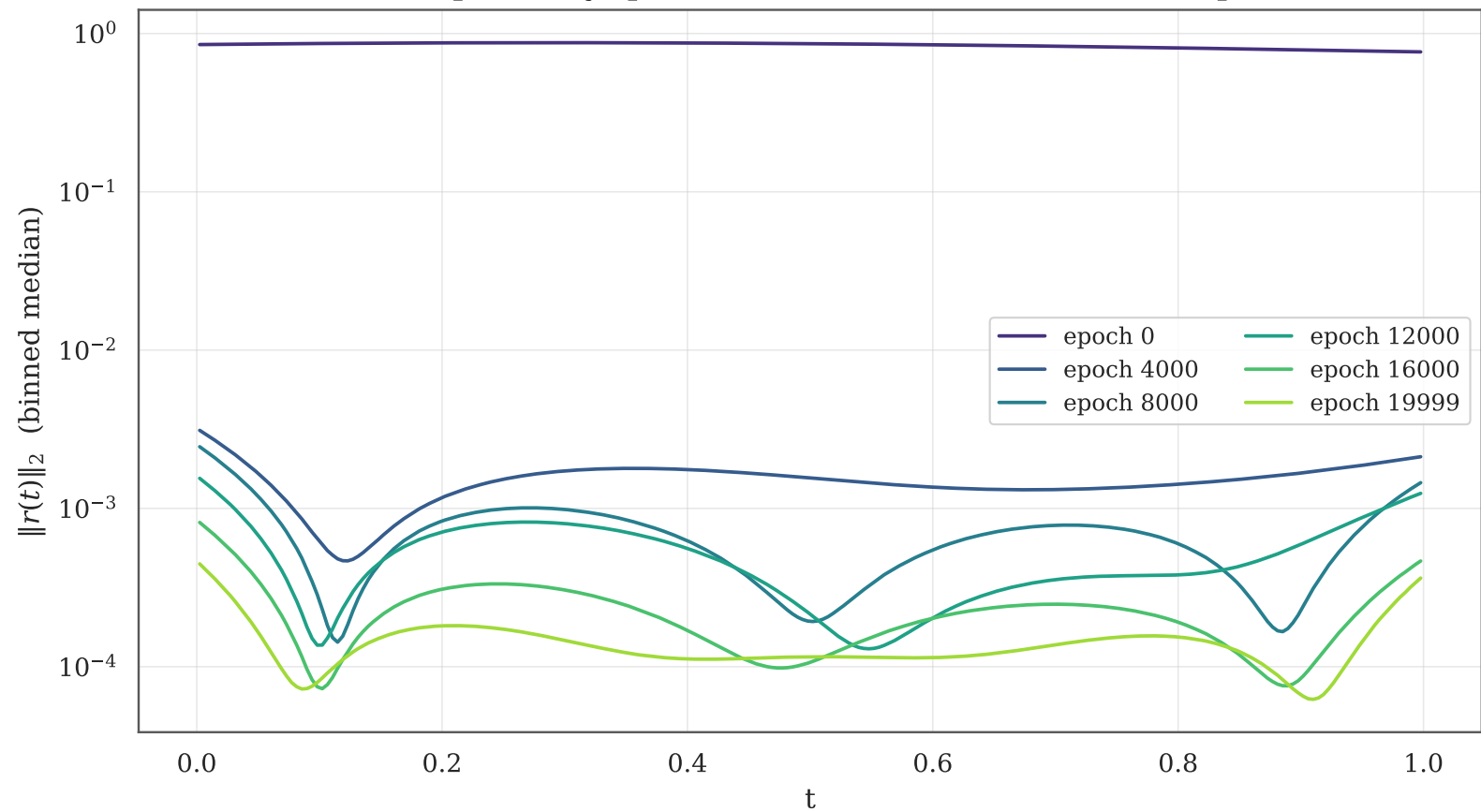
Residual profile by epoch — 4x70 tanh, hard IC, 3000 LHS points
