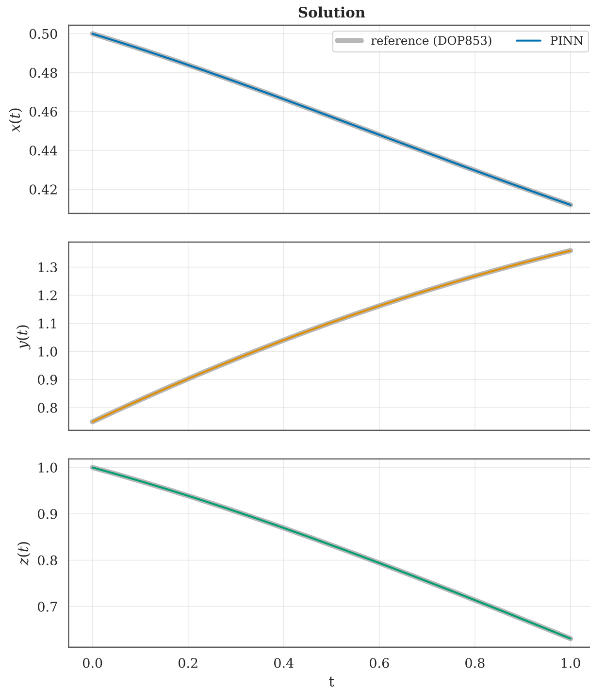
PINN solution vs reference — 4x70 tanh, hard IC, 3000 LHS points
