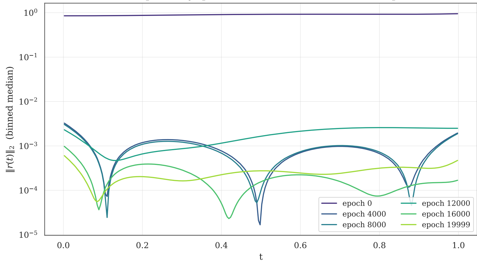
Residual profile by epoch — 5x50 tanh, hard IC, 3000 LHS points
