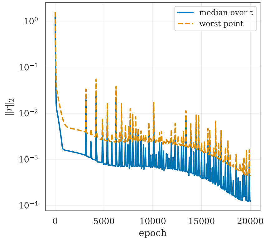
(b) Spread across collocation points
