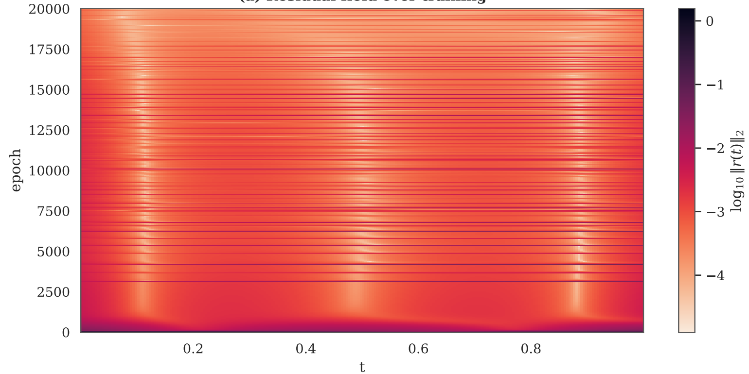
(a) Residual field over training
