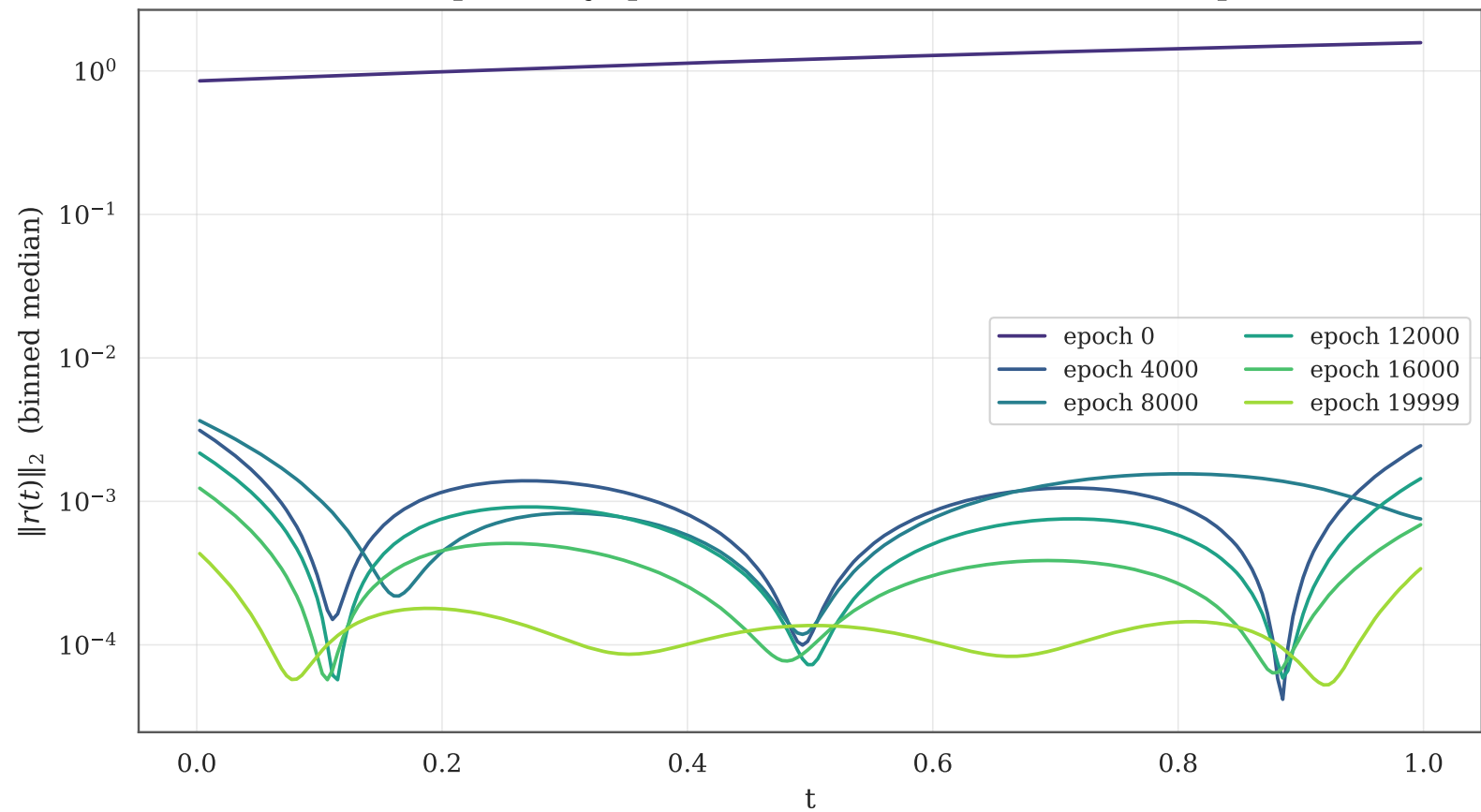
Residual profile by epoch — 5x60 tanh, hard IC, 3000 LHS points
