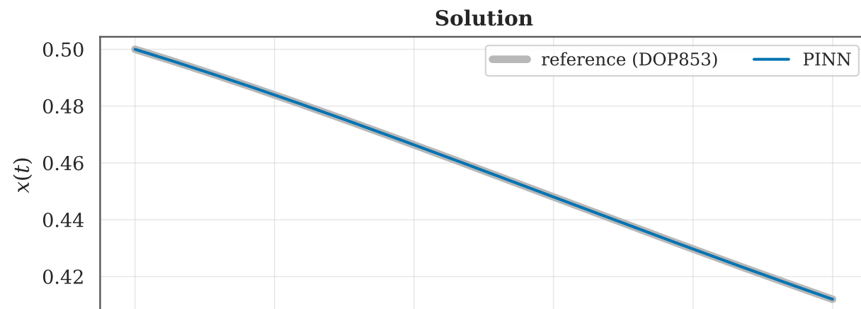
PINN solution vs reference — 5x60 tanh, hard IC, 3000 LHS points
