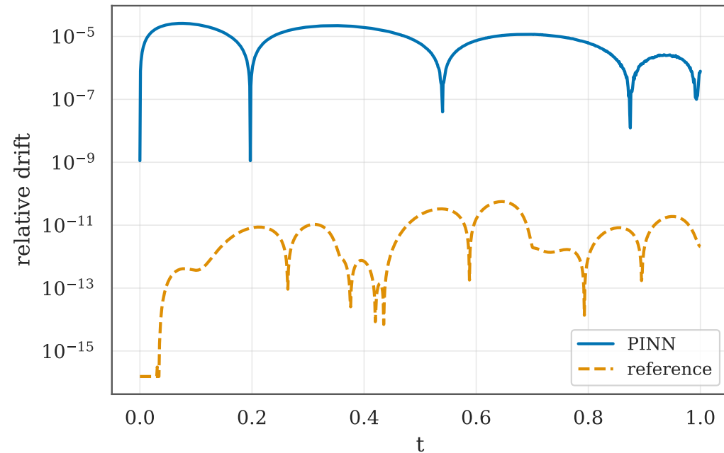
I_1 weights (+0.904, +0.226, +0.363)
