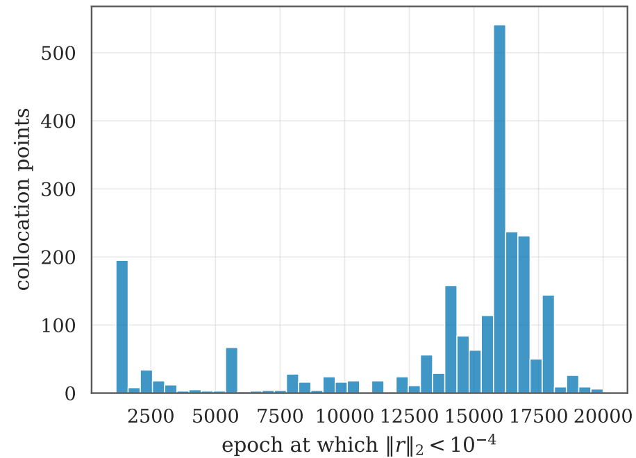
(a) Convergence epoch (723 never reached)
