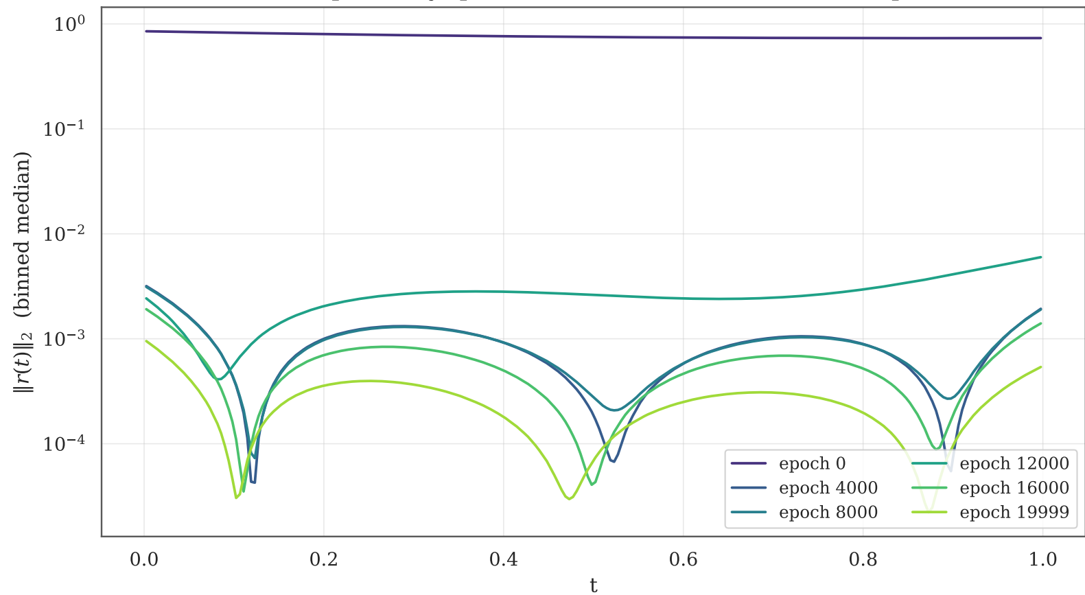
Residual profile by epoch — 3x70 tanh, hard IC, 3000 LHS points
