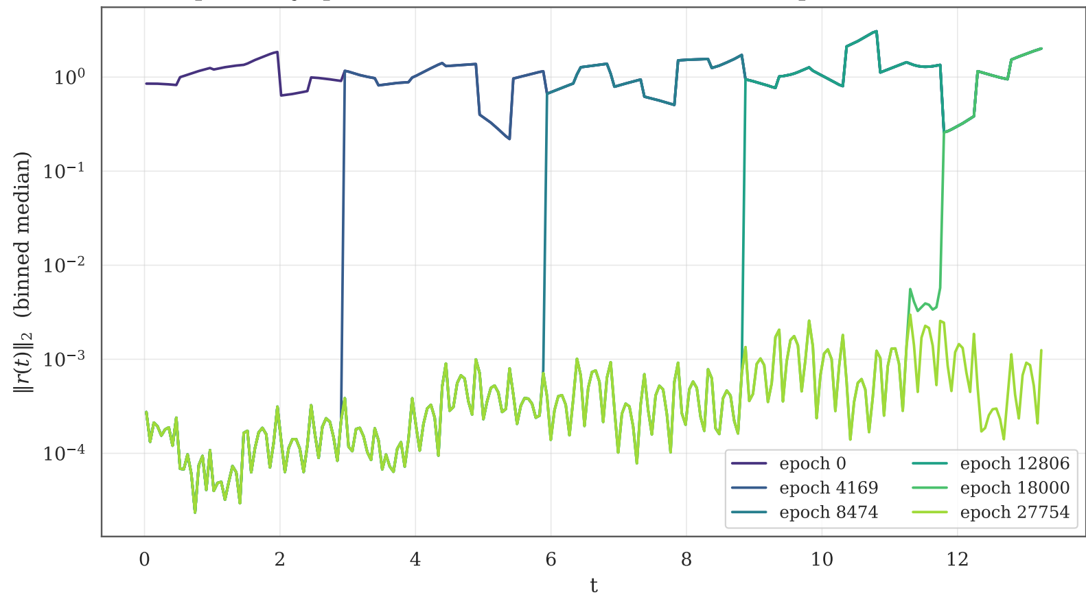
Residual profile by epoch — 4x60 tanh, hard IC, 1500 uniform points, 27 windows, causal
