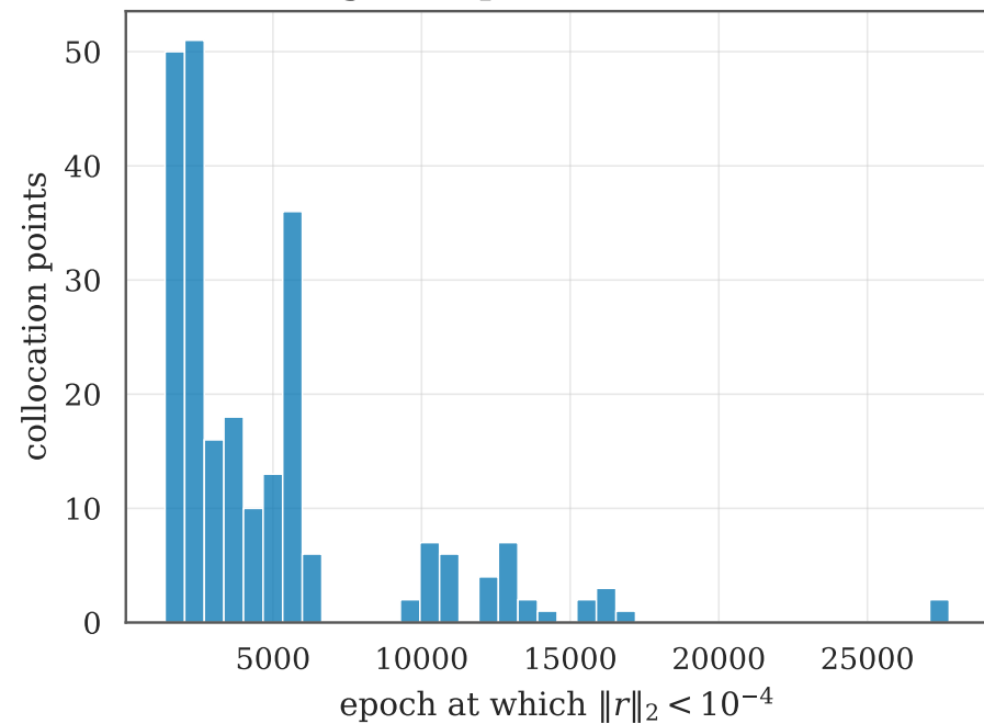
(a) Convergence epoch (1263 never reached)
