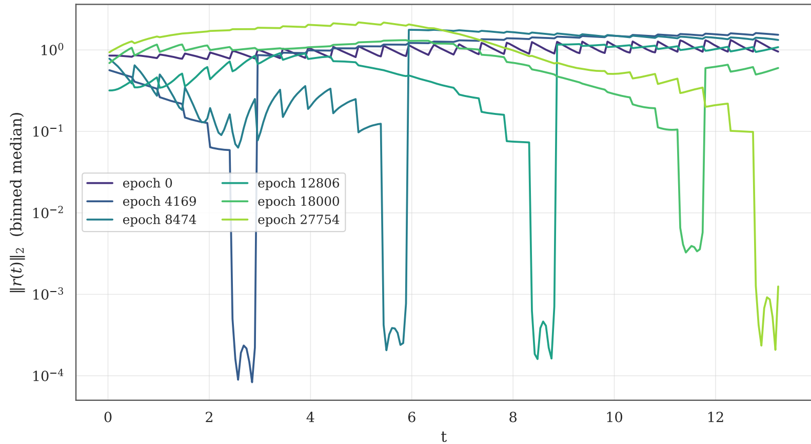
Residual profile by epoch — 4x60 tanh, hard IC, 1500 uniform points, 27 windows, shared net, causal
