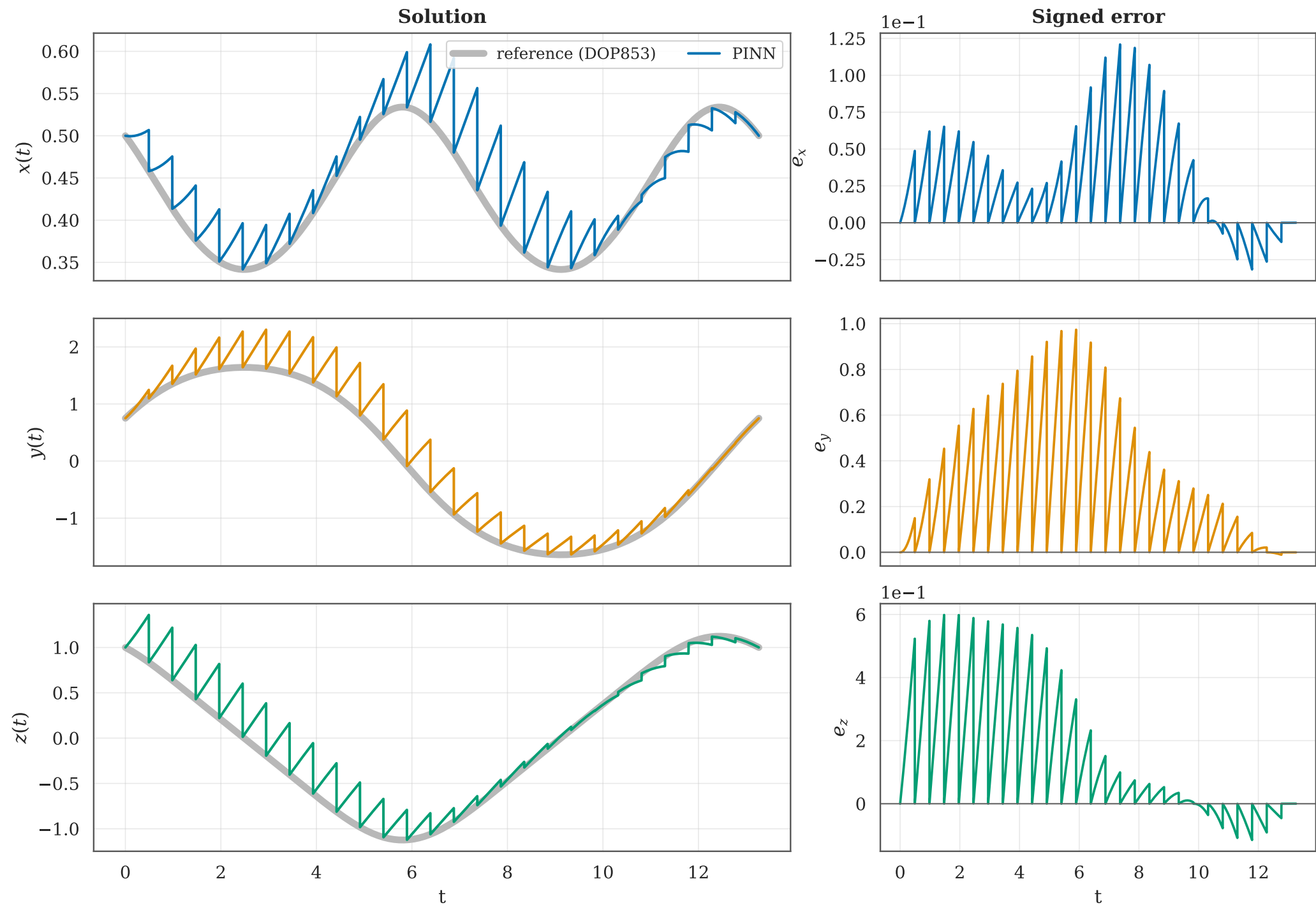
PINN solution vs reference — 4x60 tanh, hard IC, 1500 uniform points, 27 windows, shared net, causal
