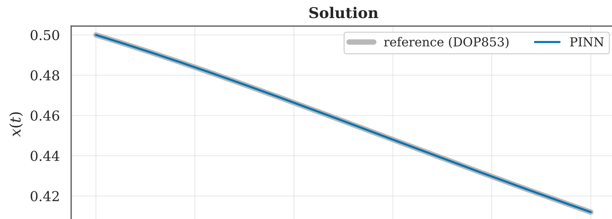
PINN solution vs reference — 5x70 tanh, hard IC, 3000 LHS points
