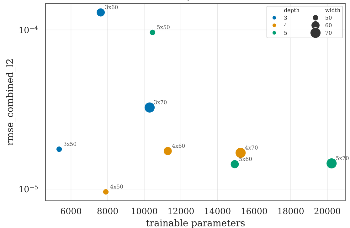
(a) Accuracy vs model size
