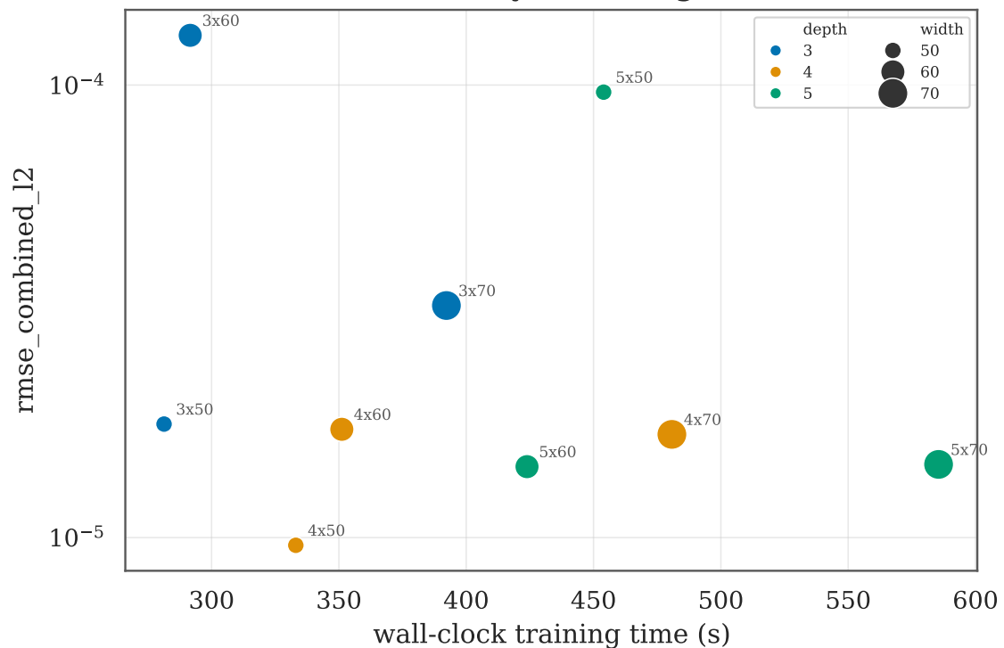
(b) Accuracy vs training cost
