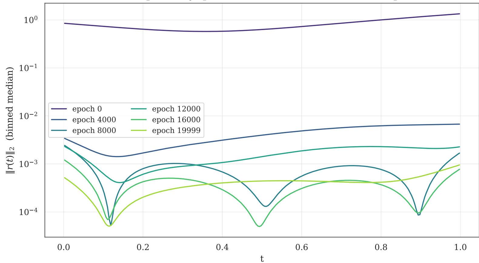
Residual profile by epoch — 3x60 tanh, hard IC, 3000 LHS points
