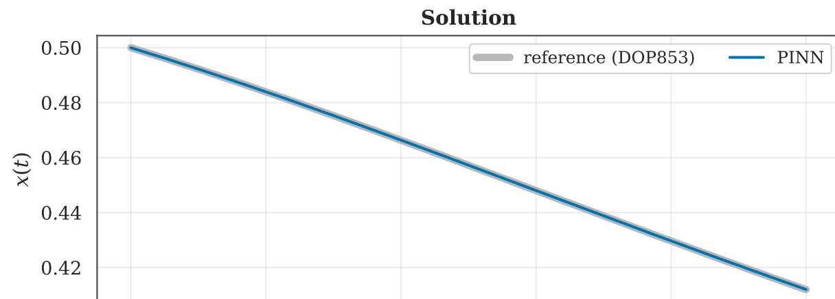
PINN solution vs reference — 3x60 tanh, hard IC, 3000 LHS points
