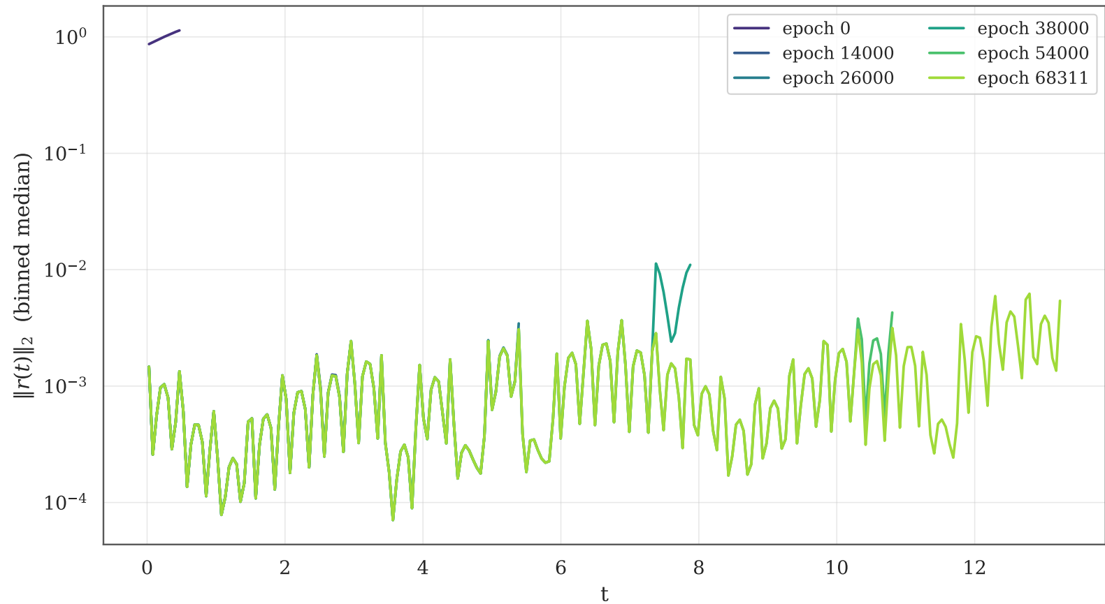
Residual profile by epoch — 4x60 tanh, hard IC, 41446 uniform points, 27 windows
