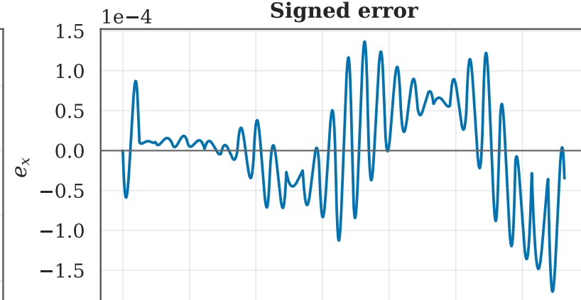
PINN solution vs reference — 4x60 tanh, hard IC, 41446 uniform points, 27 windows
