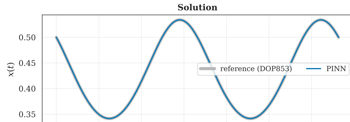
PINN solution vs reference — 4x60 tanh, hard IC, 41446 uniform points, 27 windows, causal
