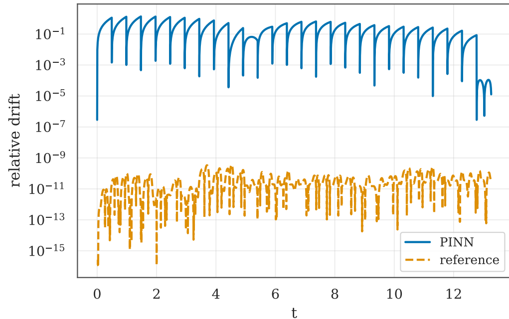
I_2 weights (-0.424, +0.363, +0.830)
