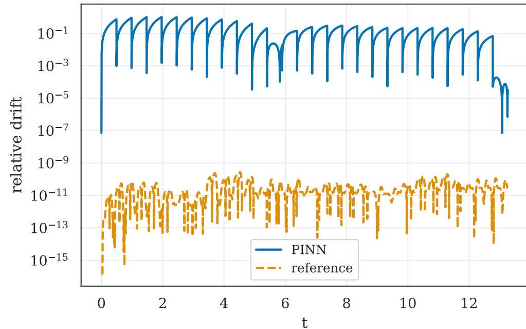
I_1 weights (+0.904, +0.226, +0.363)
