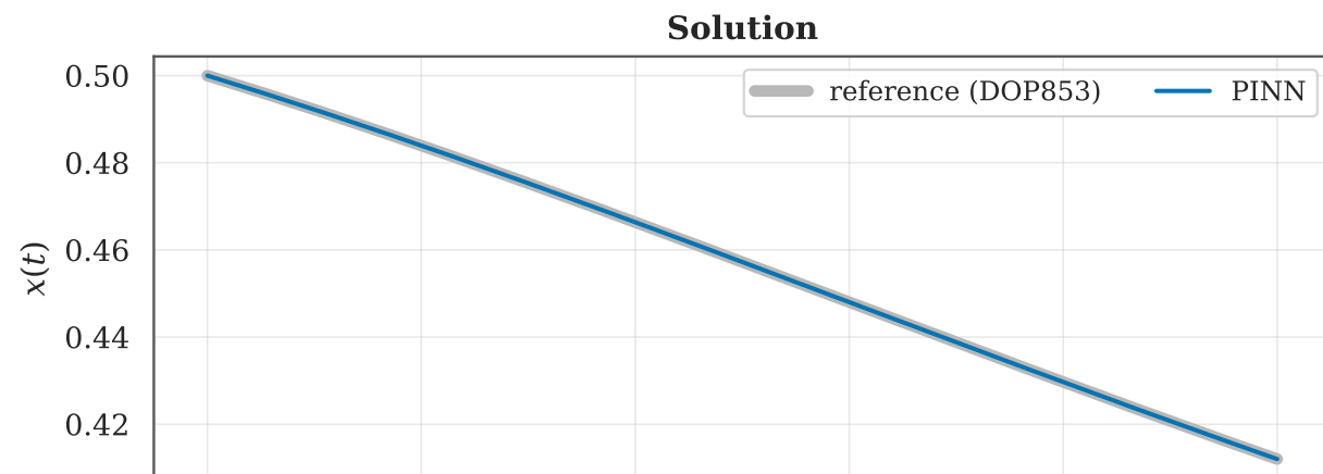
PINN solution vs reference — 4x50 tanh, hard IC, 3000 LHS points
