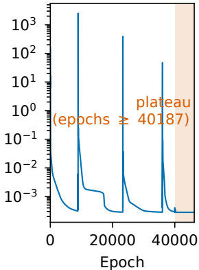
Training loss
