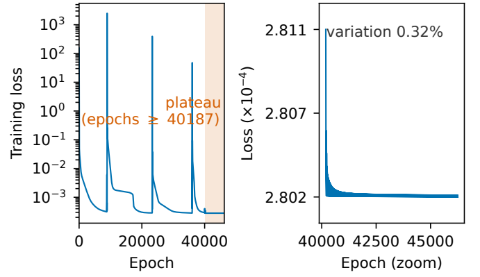
Fig. 1. Single-network training on the full interval: the ODE-residual loss plateaus near 2.8 \times 10^{-4} (shaded) over the final \sim 6,000 epochs, so late-time error remains large.
