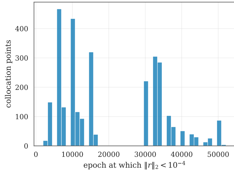
(a) First observed threshold crossing (10827 never reached)
