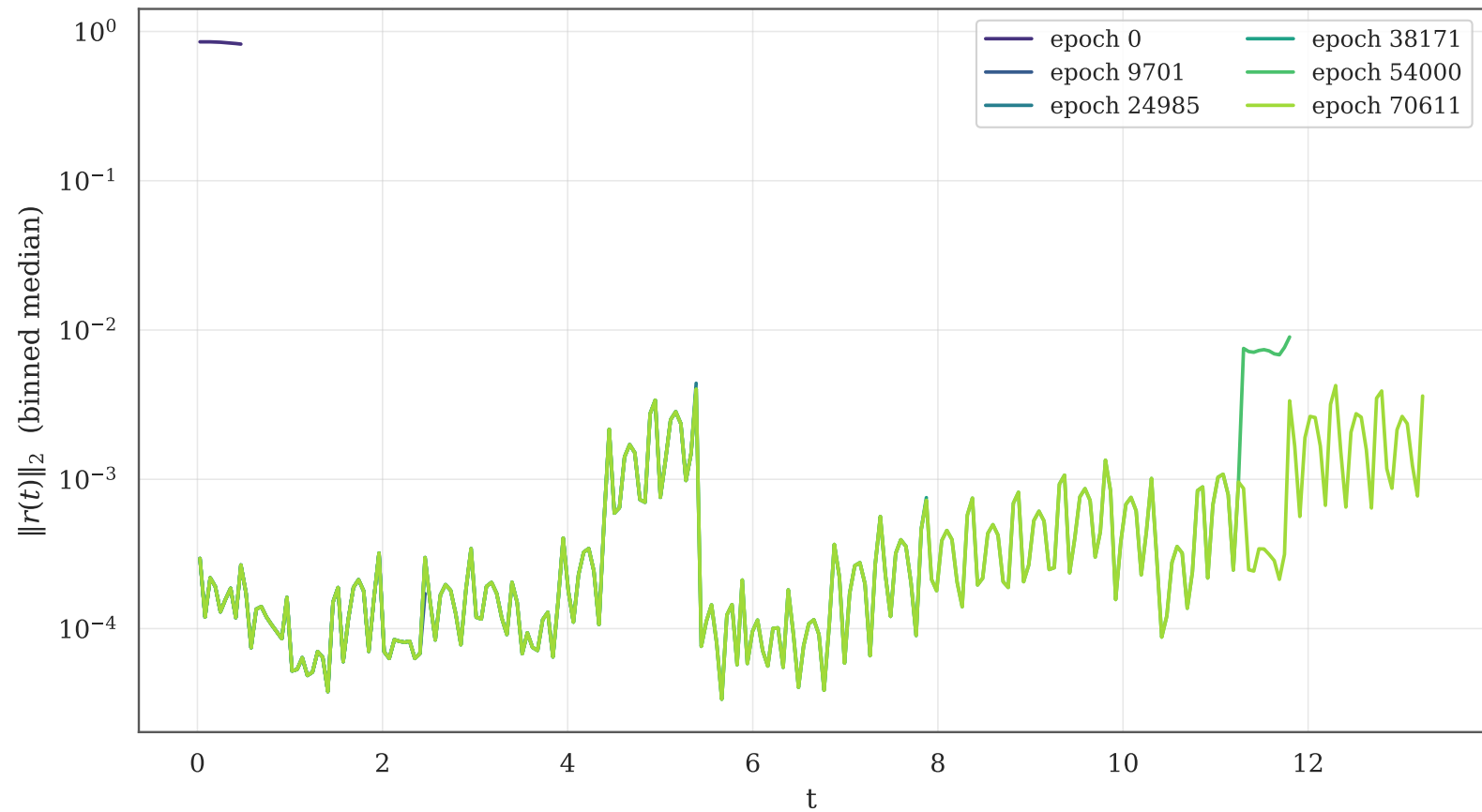
Residual profile by epoch — 4x60 tanh, hard IC, 13825 uniform points, 27 windows, causal
