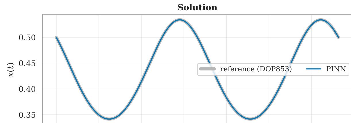
PINN solution vs reference — 4x60 tanh, hard IC, 13825 uniform points, 27 windows, causal
