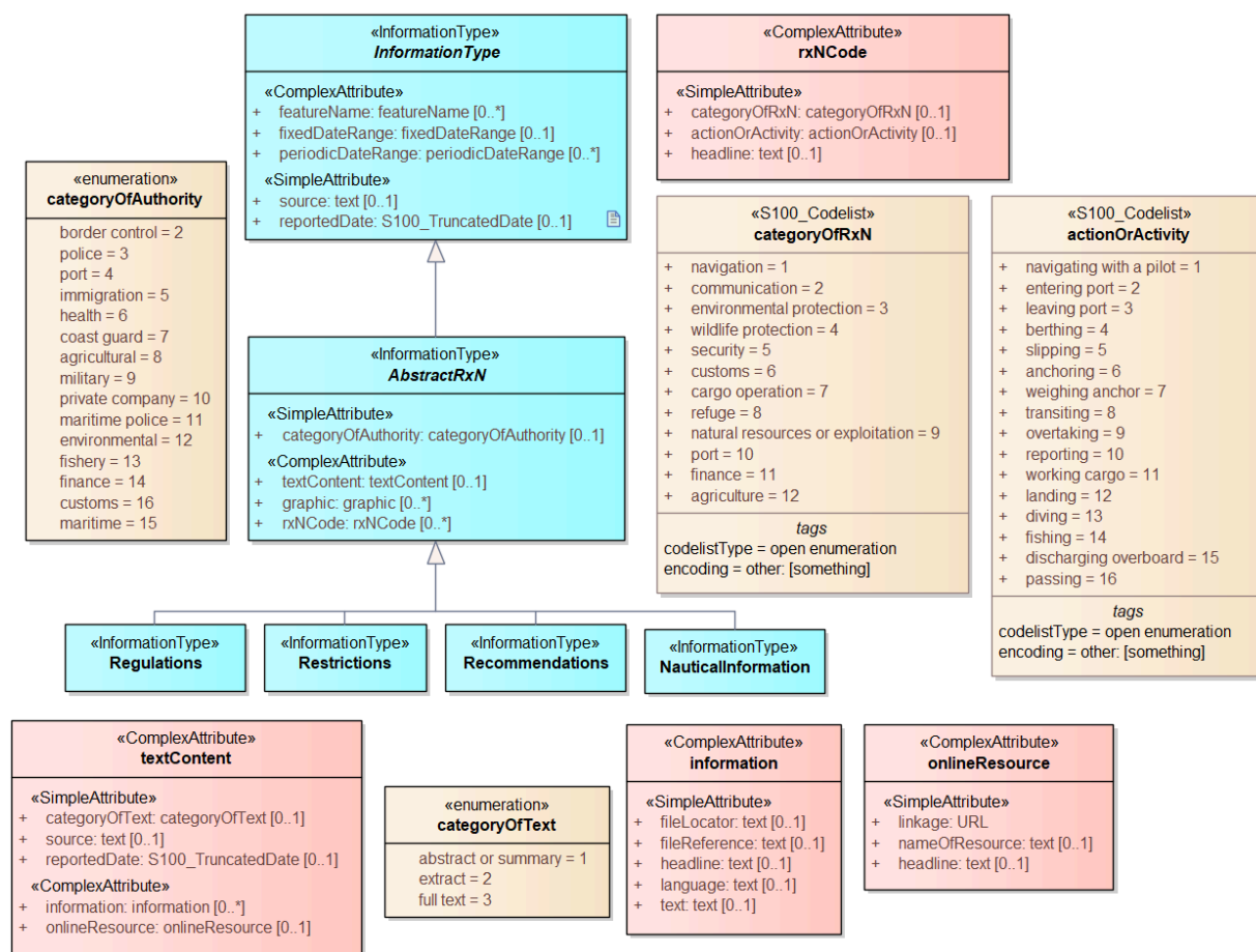
Figure 4-19 — Regulations, etc., relevant to specific features
