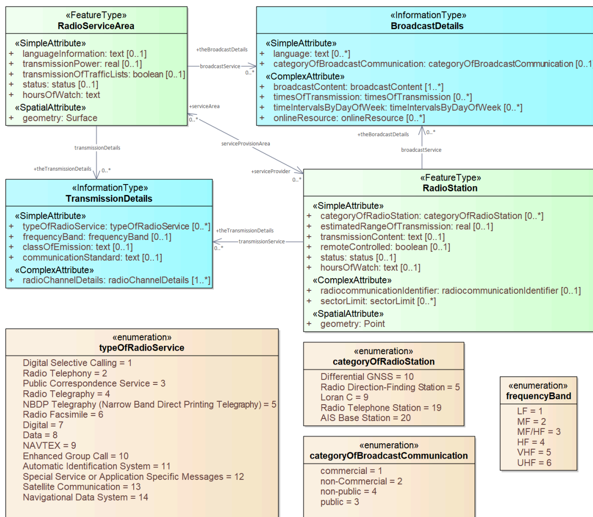
Figure 4-9 — RadioServiceArea for encoding various type of services
