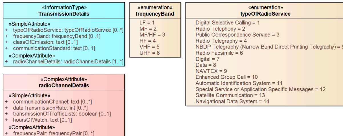
Figure 4-5 — The TransmissionDetails information type
