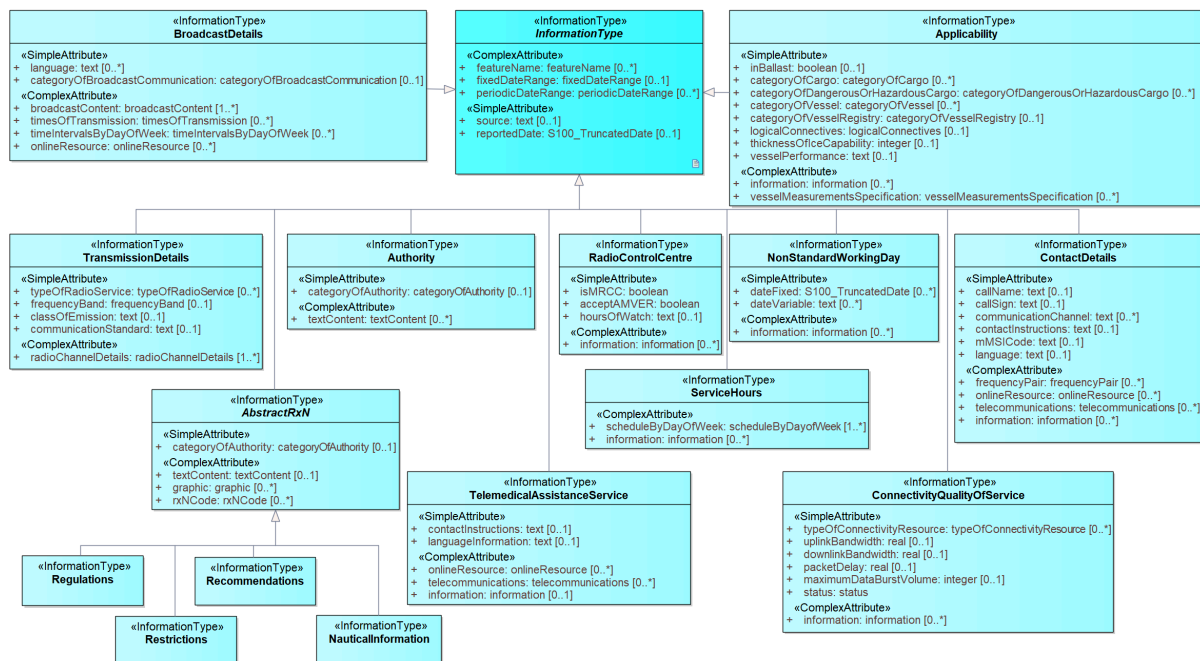
Figure 4-3 — Overview of S-123 Information Types
