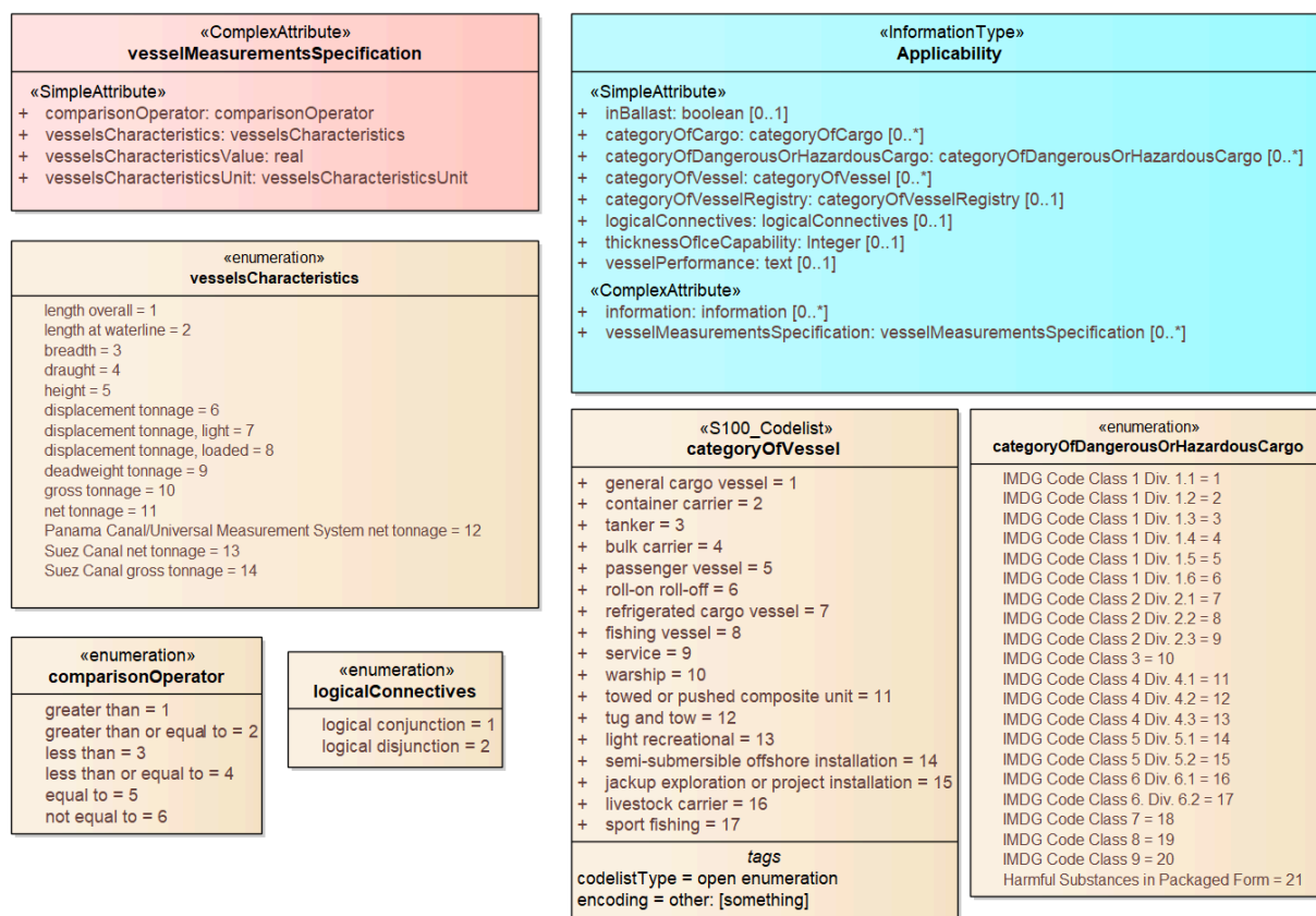
Figure 4-21 — Applicability of requirements, rules, etc. to vessel categories
