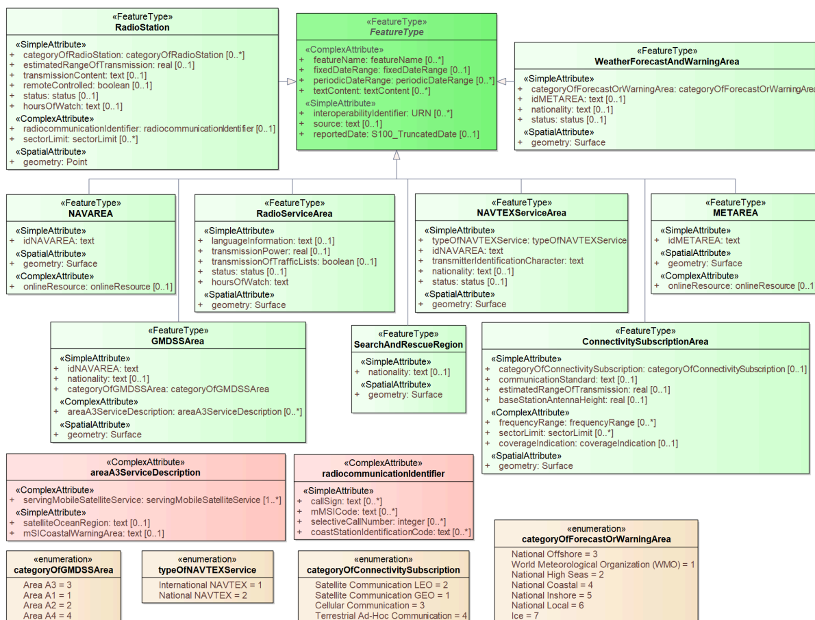
Figure 4-2 — Overview of S-123 Feature Types
