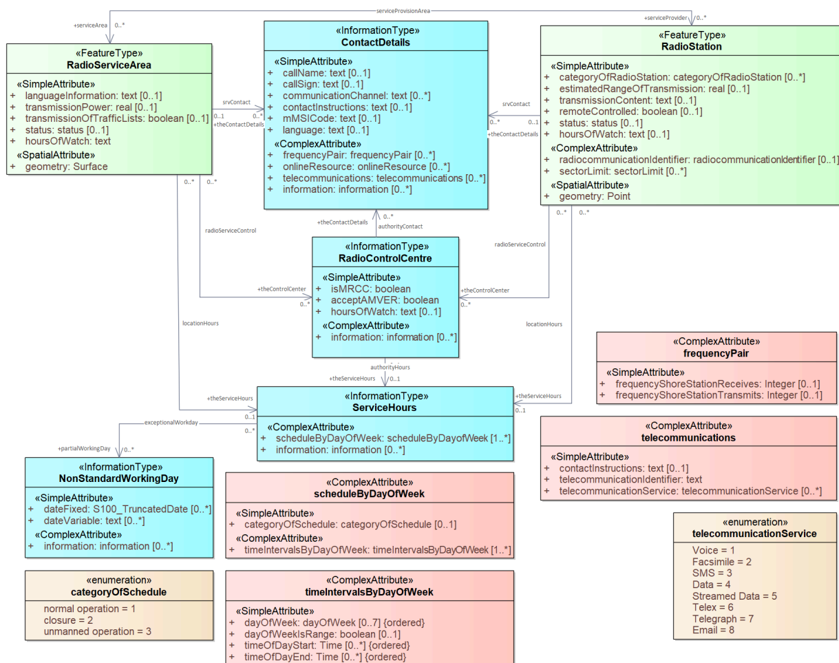
Figure 4-7 — S-123 Radio service features with contact information and service hours
