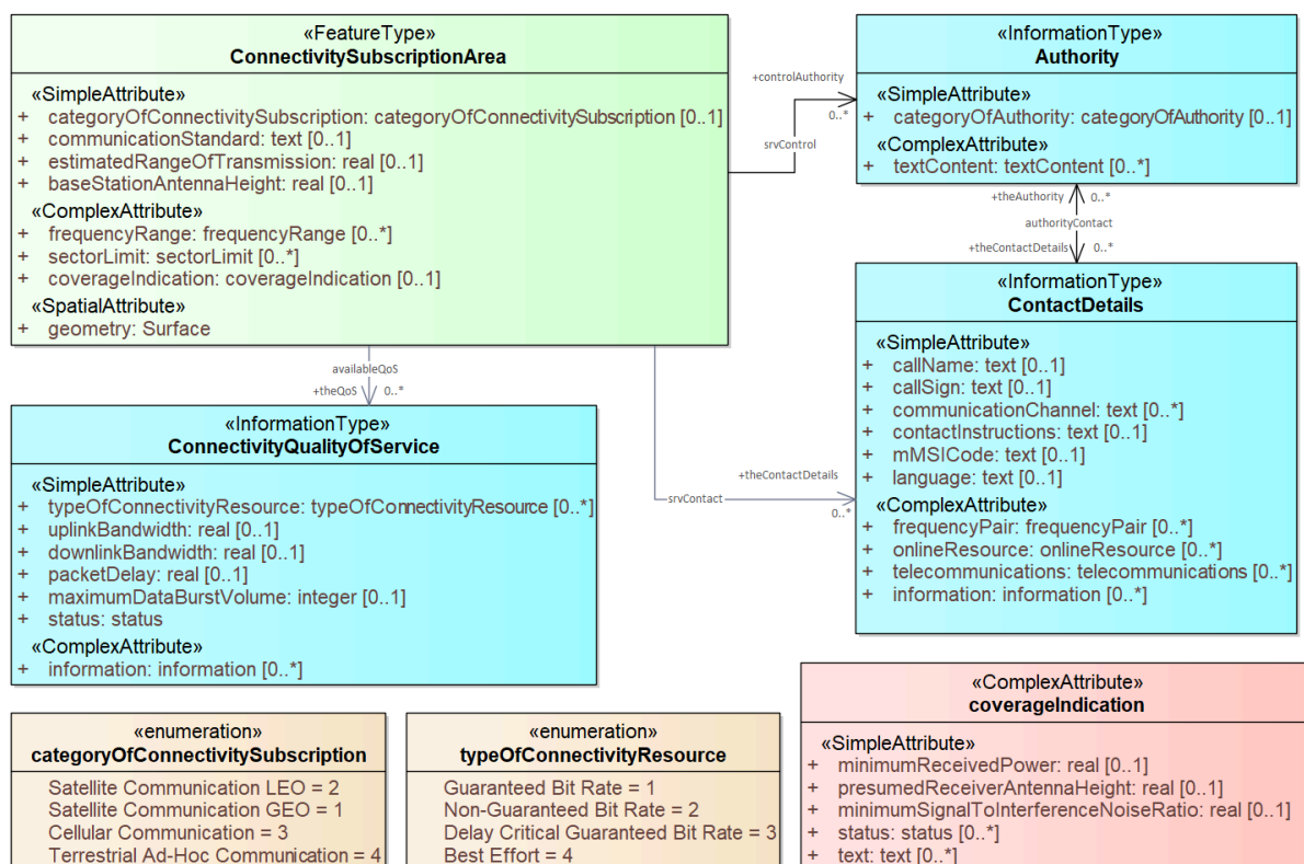
Figure 4-15 — Connectivity subscription area
