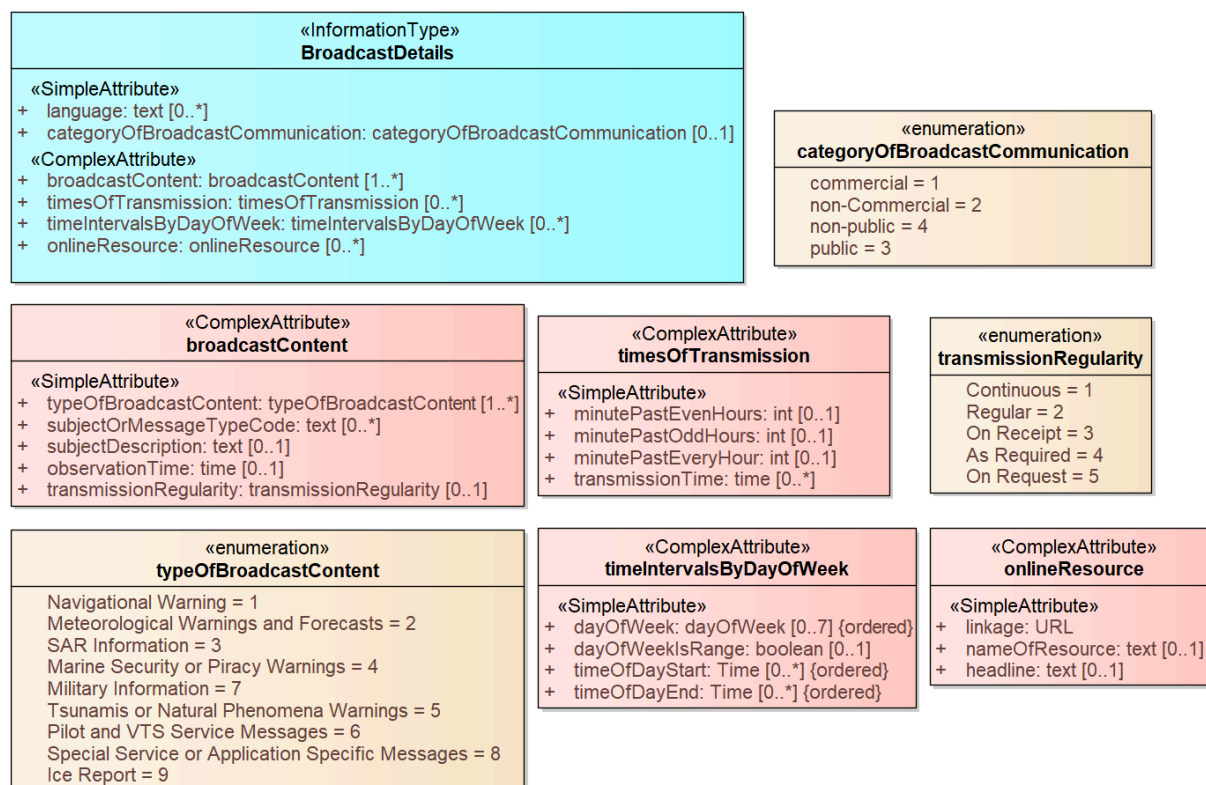
Figure 4-6 — The BroadcastDetails information type
