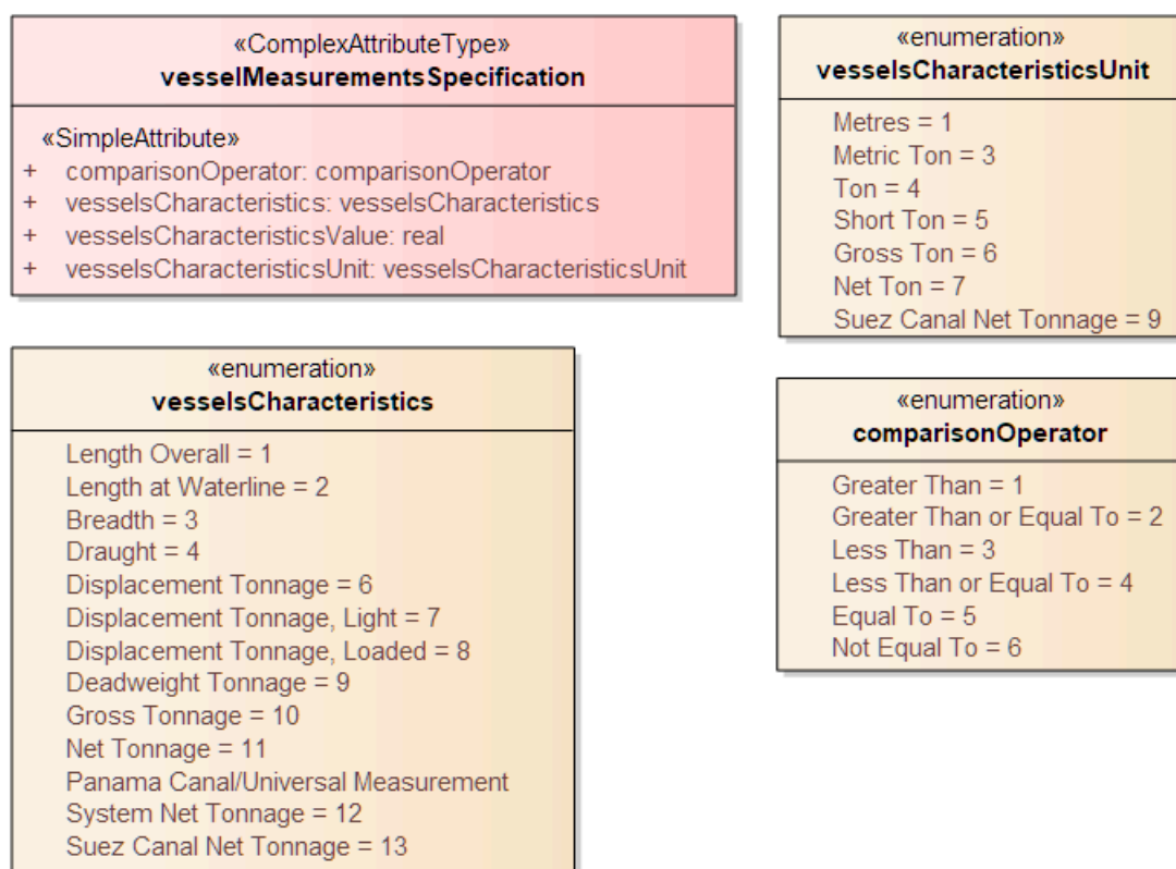
Figure 15-2 — Attributes for specifying vessel dimensions
