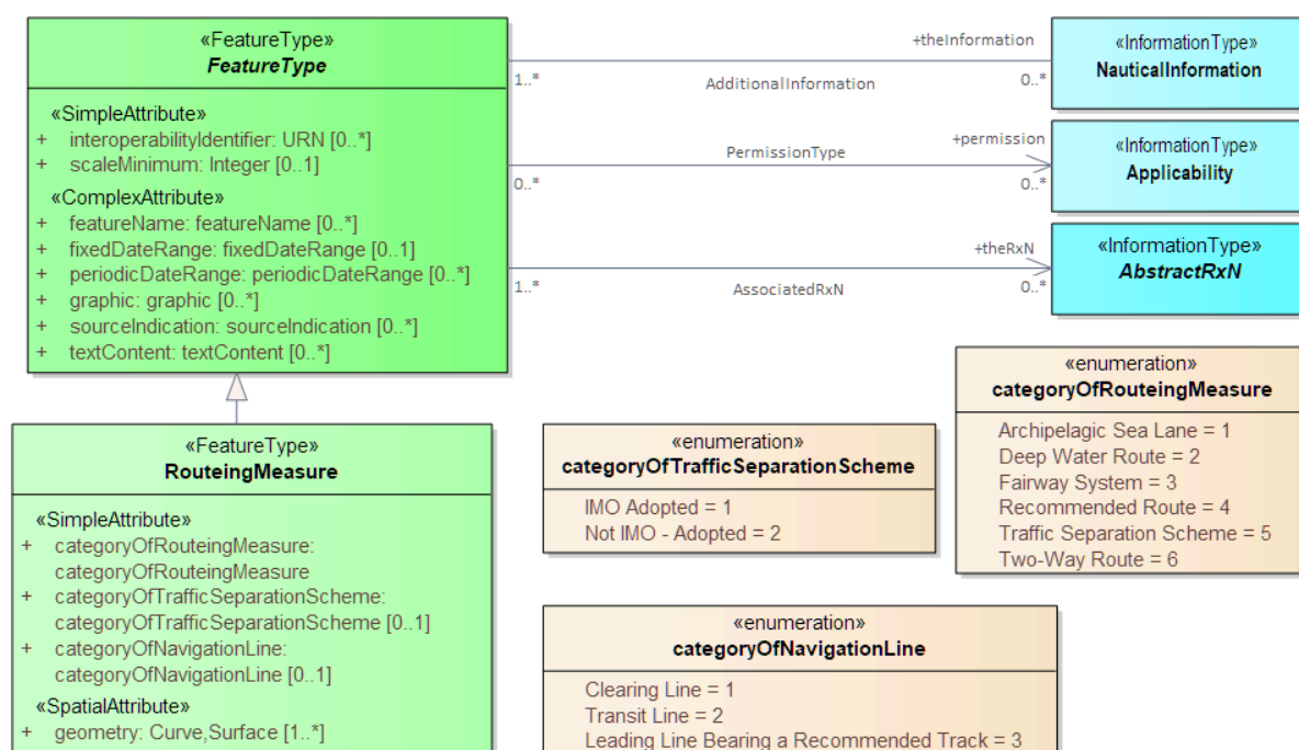
Figure 6-1 — Routeing measures model
