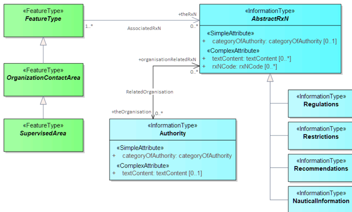
Figure 13-2 — Regulations, etc., for geo features
