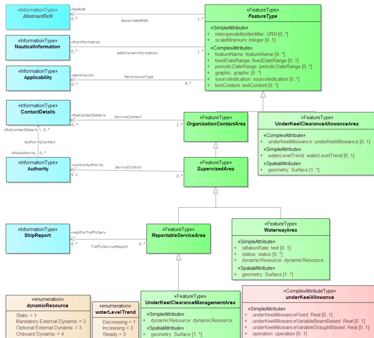
Figure 8-1 — Underkeel clearances
