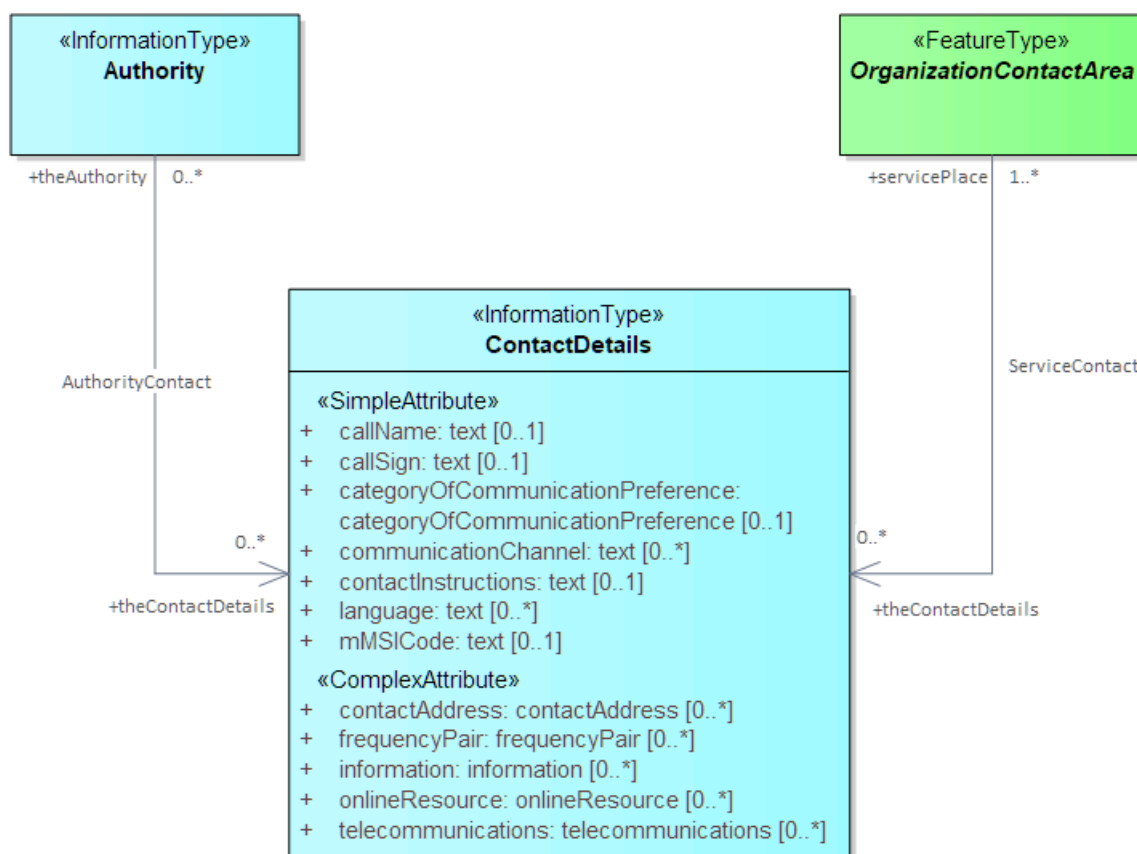
Figure 14-2 — Associations to contact information
