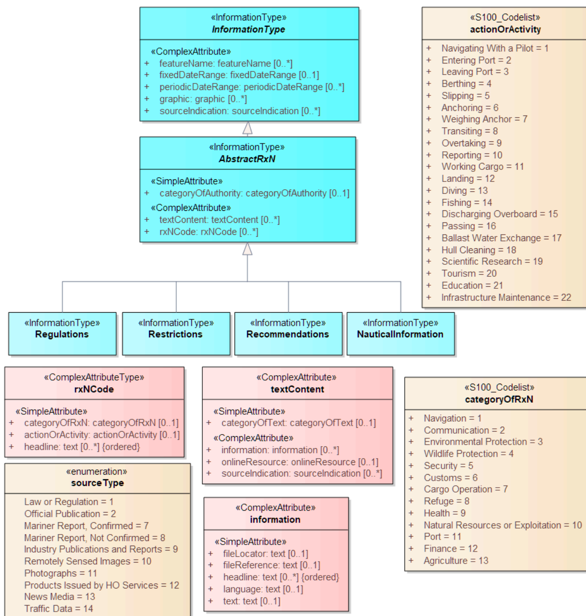
Figure 13-1 — Types for textual information concerning regulations, etc.
