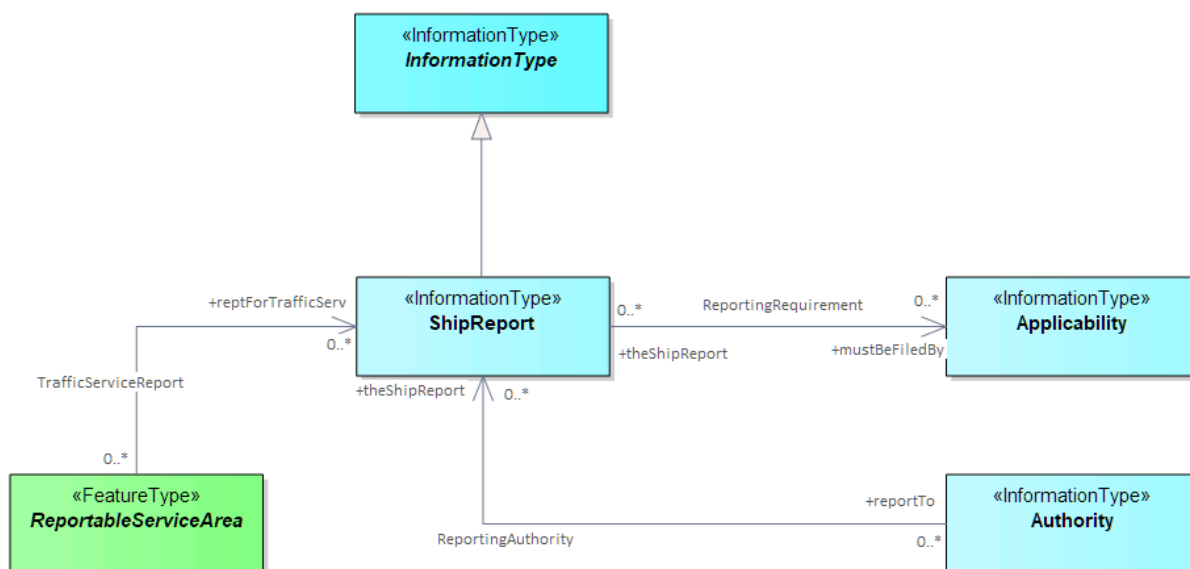
Figure 16-1 — ShipReport and related types.
