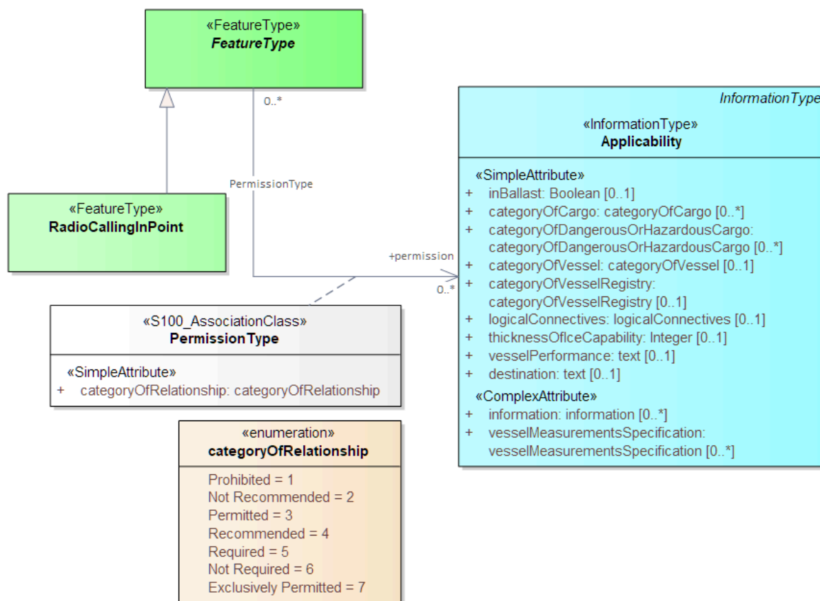
Figure 2-3 — Association class for hypothetical requirement for use of a radio calling-in point by a vessel carrying hazardous cargo
