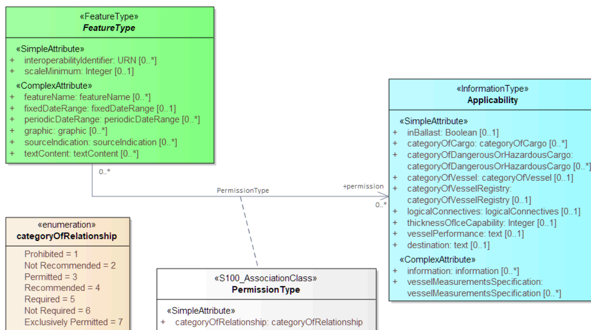
Figure 2-4 — Association class for inclusion of vessel types in regulations
