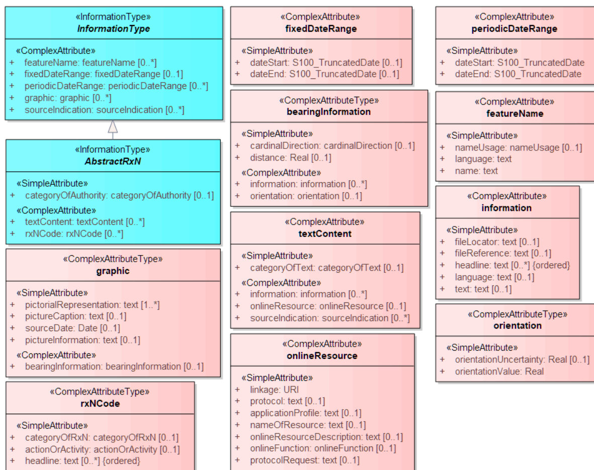
Figure 12-1 — Abstract Information Types
