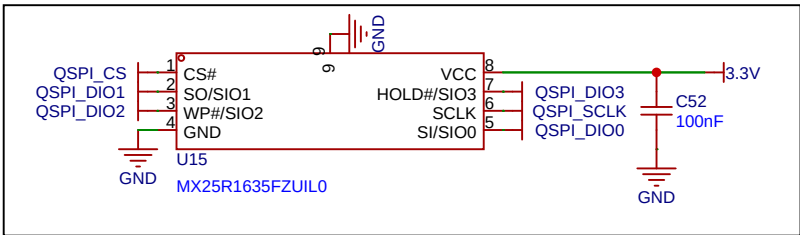
FLASH_MEMORY
