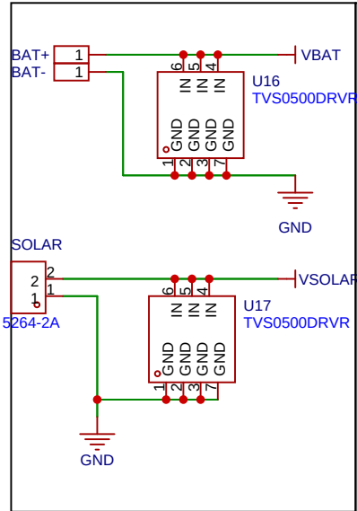
POWER_PORT
