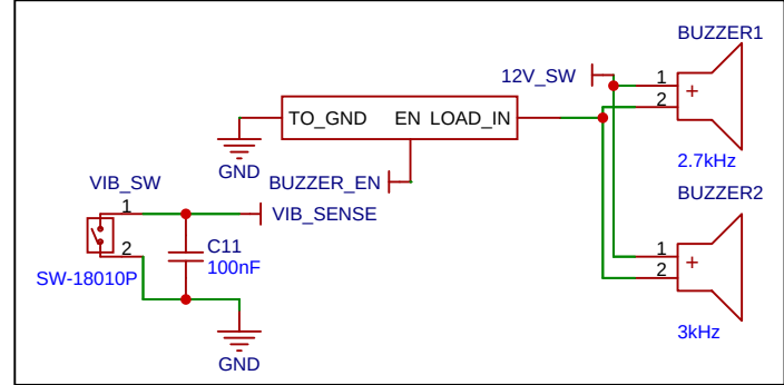
ANTI_THEIF
