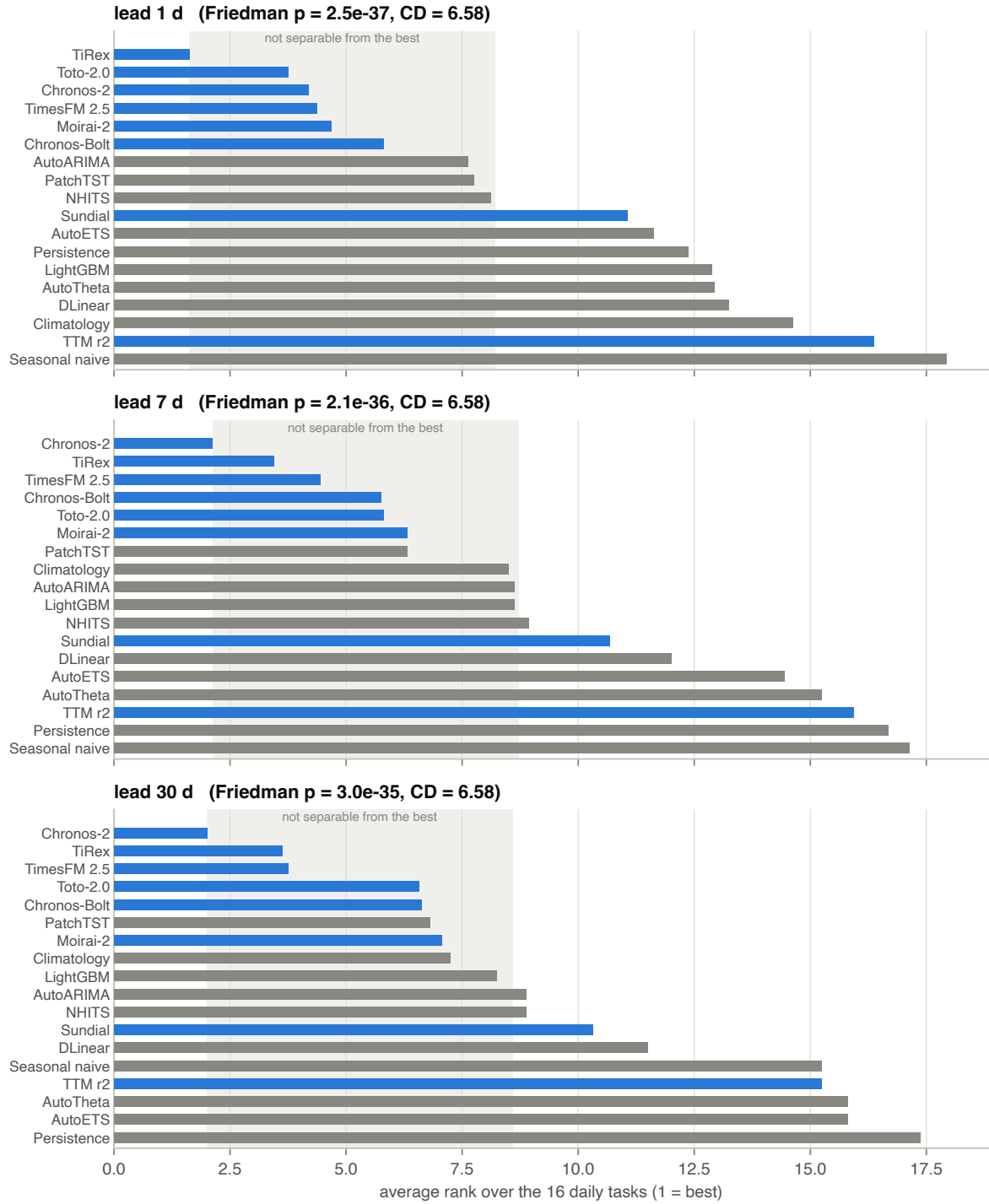
Figure 1: Average rank over the 16 daily tasks, with the shaded band marking one Nemenyi critical difference from the best model. Foundation models in blue, baselines in grey. The leading group is not internally separable.
