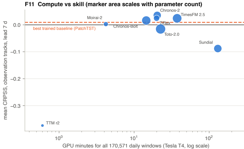
Figure 4: Compute against skill on the observation tracks at a 7-day lead; marker area scales with parameter count. The full leaderboard is reproducible in roughly four GPU-hours on free hardware.
