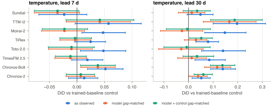
Figure 3: Difference-in-differences against the trained-baseline control, with 95% intervals. Positive values mean the model loses more skill in the tropics than the control does. Masking the control as well as the model is the like-for-like comparison.
