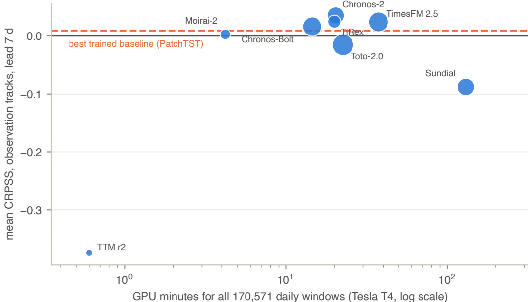
Compute vs skill (marker area scales with parameter count)
