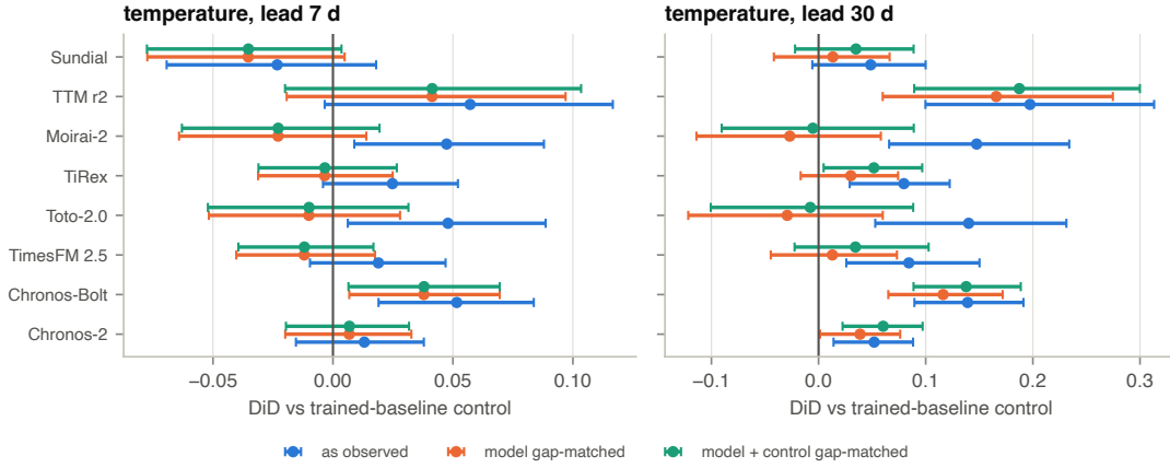
Figure 6: Difference-in-differences against the trained-baseline control, with 95% intervals. Positive values mean the model loses more skill in the tropics than the control does. Masking the control as well as the model is the like-for-like comparison.
